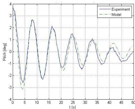
Figure 4: Pitch decaying test.
