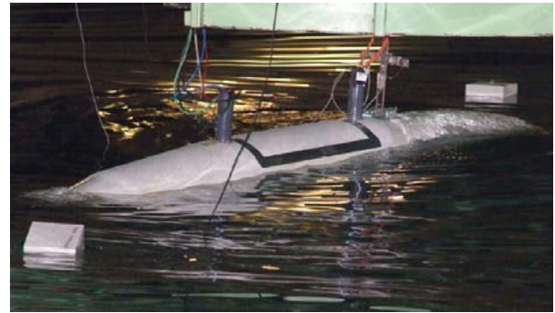
Figure 3: 1:15 scale model in wave tank test.
