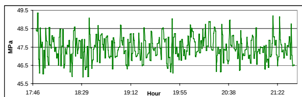
Figure 9: Record of strain gauge 5 (03/10/2008)
