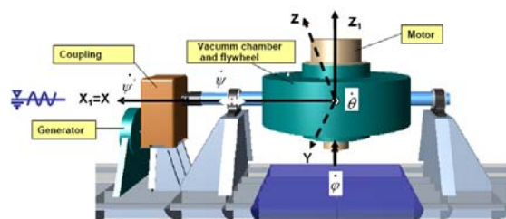
Figure 2: Functional design of the absorber system.
