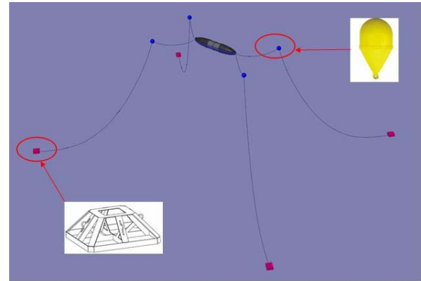
Figure 5: 3D View of the mooring system.
