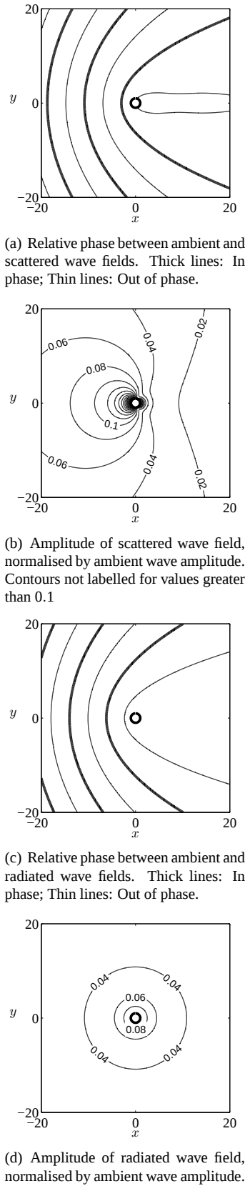
Figure 2: Radiated and scattered wave field from a real tuned isolated device for 2ak = 0.8 , \beta = 0 .
