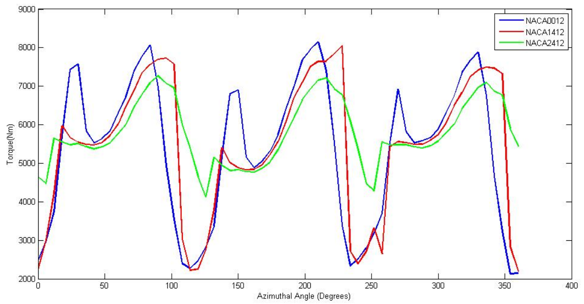
Figure 11: Darrieus Turbine: Effect of Different Cambered Blades on Shaft Torque
