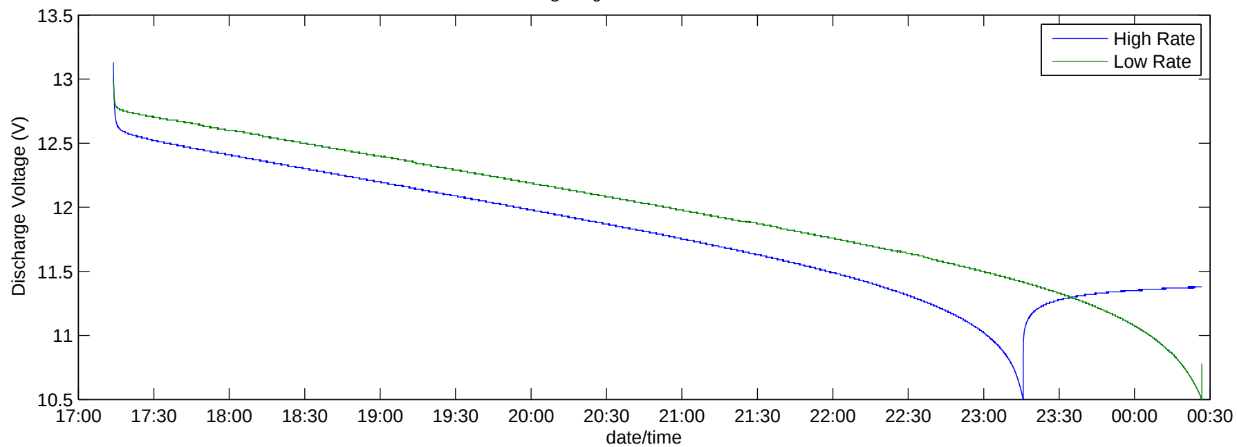
DischargeData Cycle 3 .txt Elapsed Time = 7.2142 Hrs
