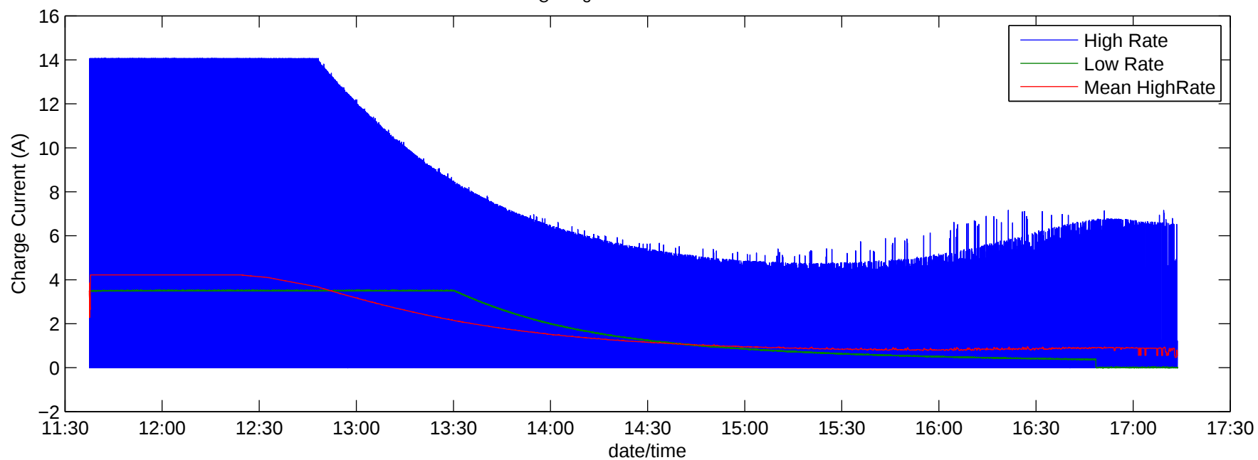
ChargeData Cycle 3 .txt Elapsed Time = 5.6047 Hrs
