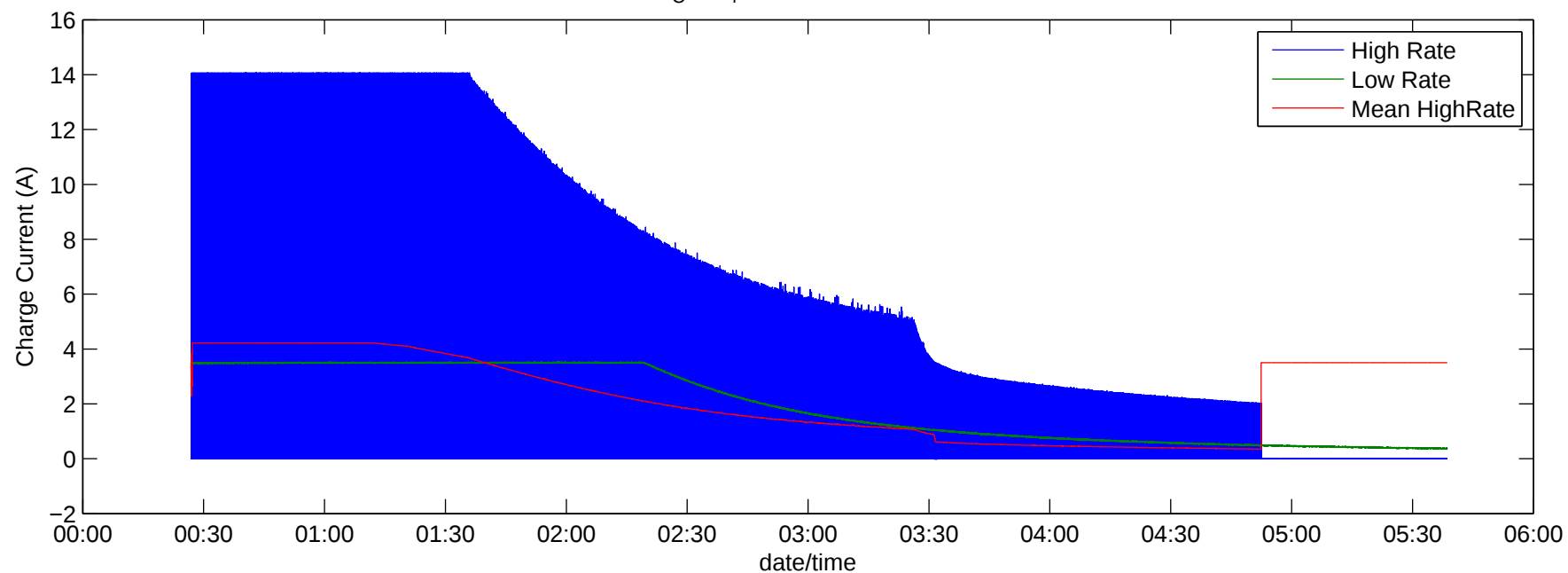
ChargeData Cycle_4 .txt Elapsed Time = 5.1956 Hrs
