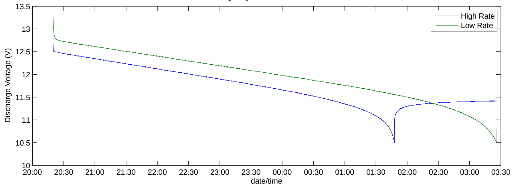
DischargeData_cycle 9 .txt Elapsed Time = 7.1044 Hrs
