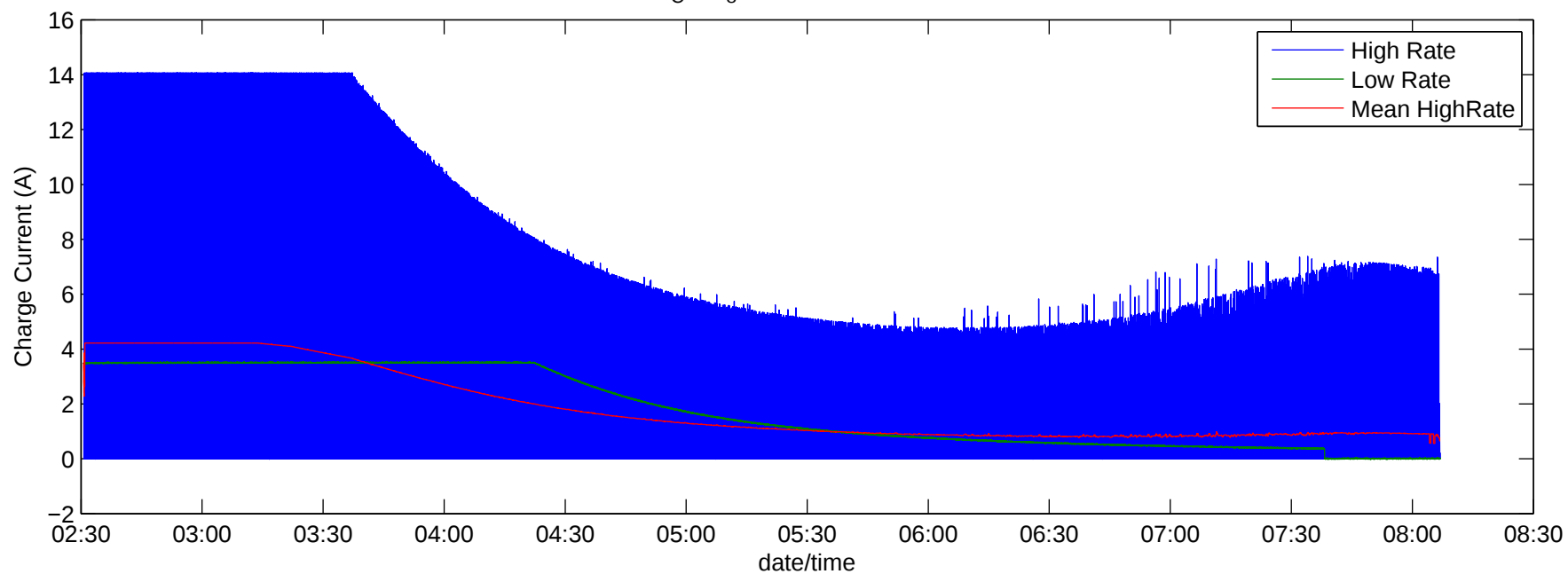
ChargeData_cycle 8 .txt Elapsed Time = 5.6047 Hrs
