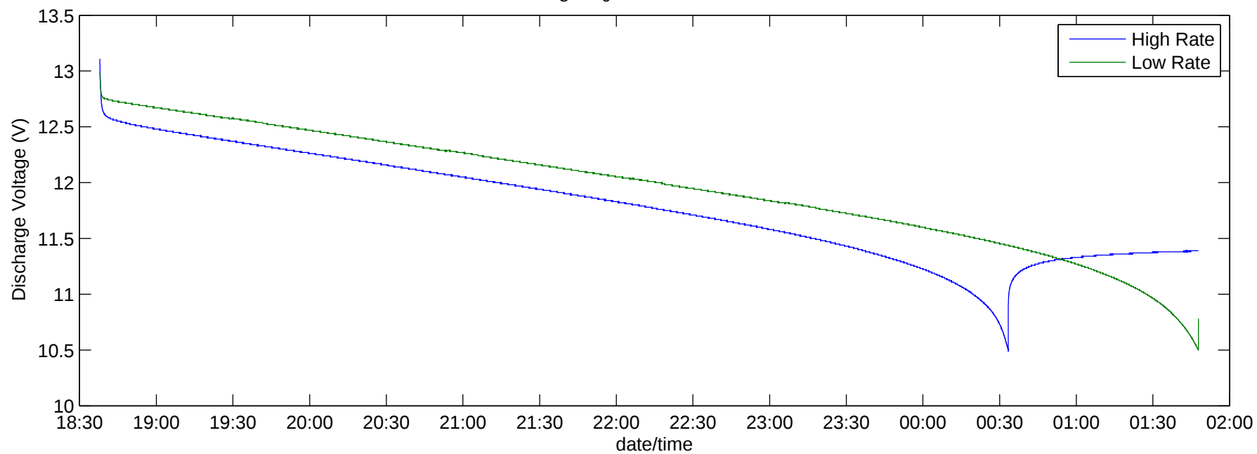
DischargeData Cycle_5 .txt Elapsed Time = 7.1653 Hrs
