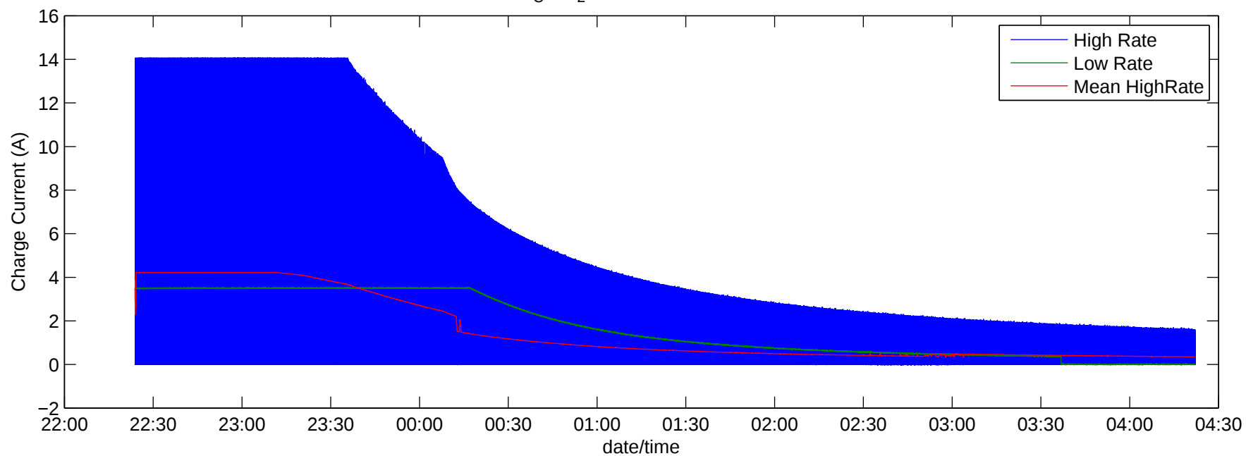
ChargeData Cycle 2 .txt Elapsed Time = 5.9728 Hrs
