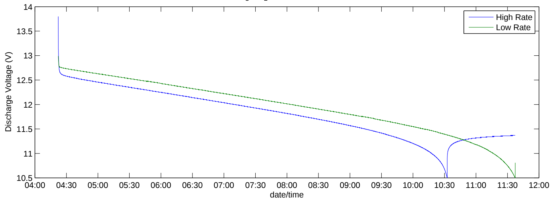
DischargeData_cycle_2.txt Elapsed Time = 7.2517 Hrs
