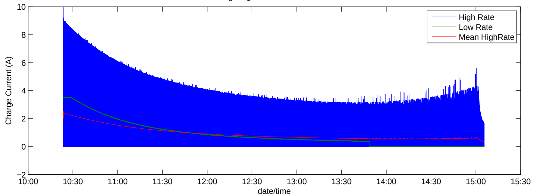
ChargeData_cycle 1 .txt Elapsed Time = 4.7019 Hrs
