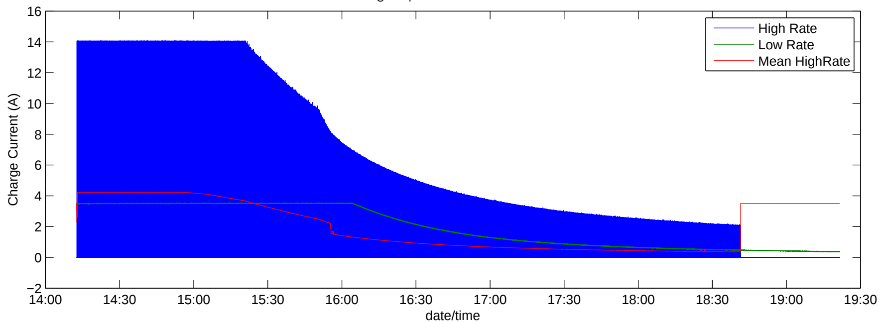
ChargeData Cycle 7 .txt Elapsed Time = 5.1492 Hrs
