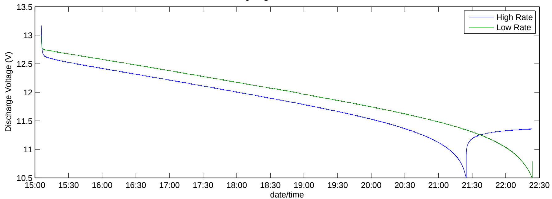
DischargeData_cycle 1 .txt Elapsed Time = 7.2997 Hrs
