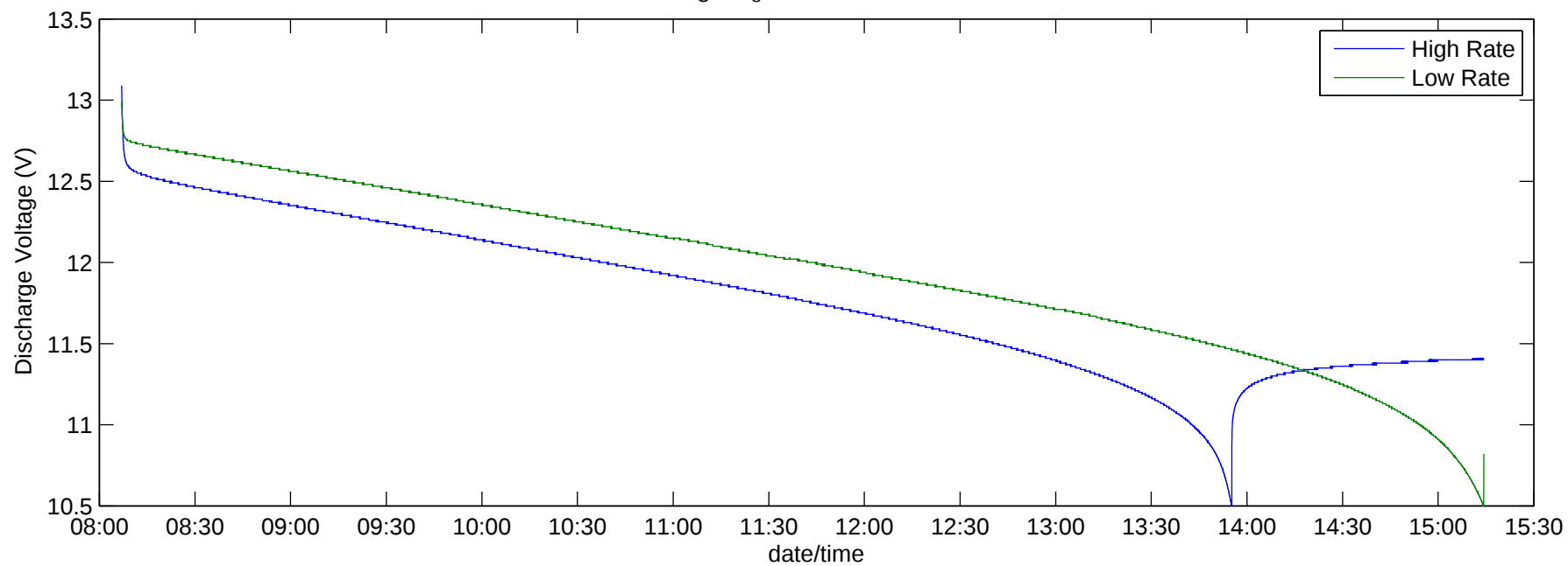
DischargeData Cycle 8 .txt Elapsed Time = 7.1217 Hrs
