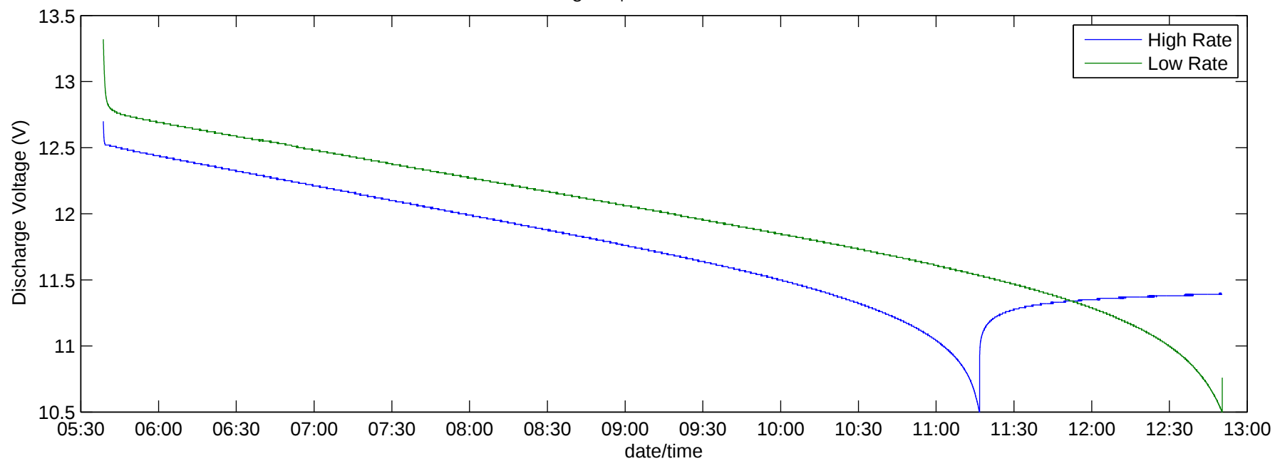
DischargeData Cycle 4 .txt Elapsed Time = 7.195 Hrs
