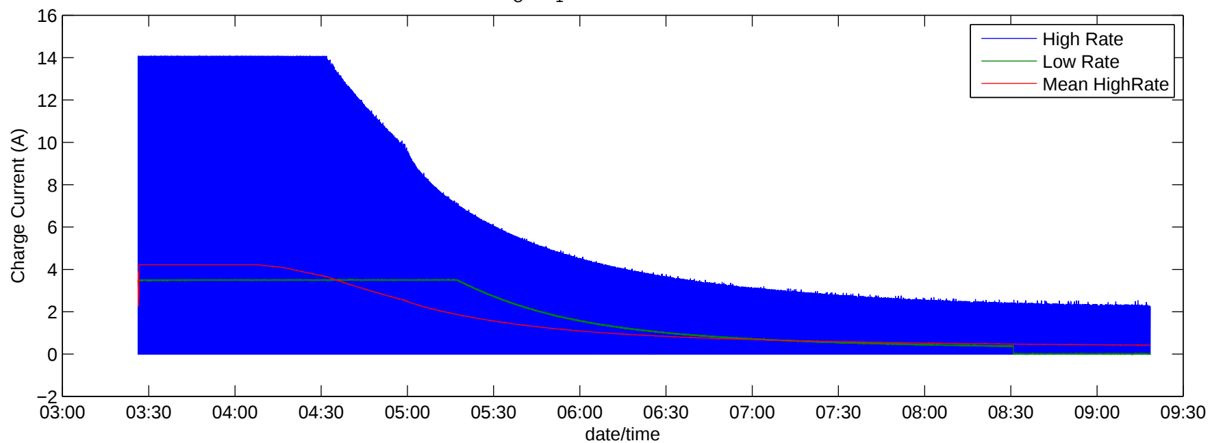
ChargeData_cycle_10.txt Elapsed Time = 5.8714 Hrs
