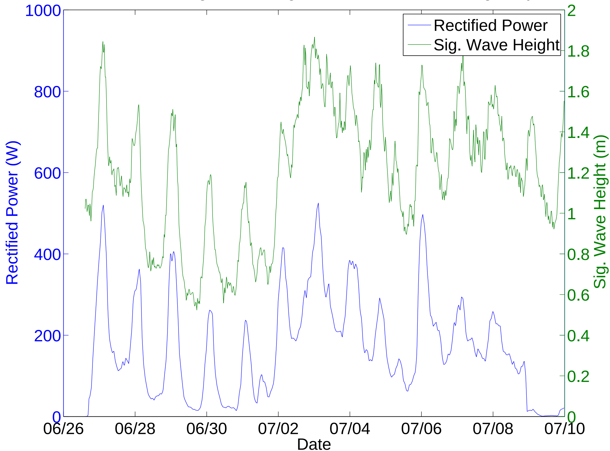
Electrical Power and Sig. Wave Height for June 26, 2012 through July 10, 2012
