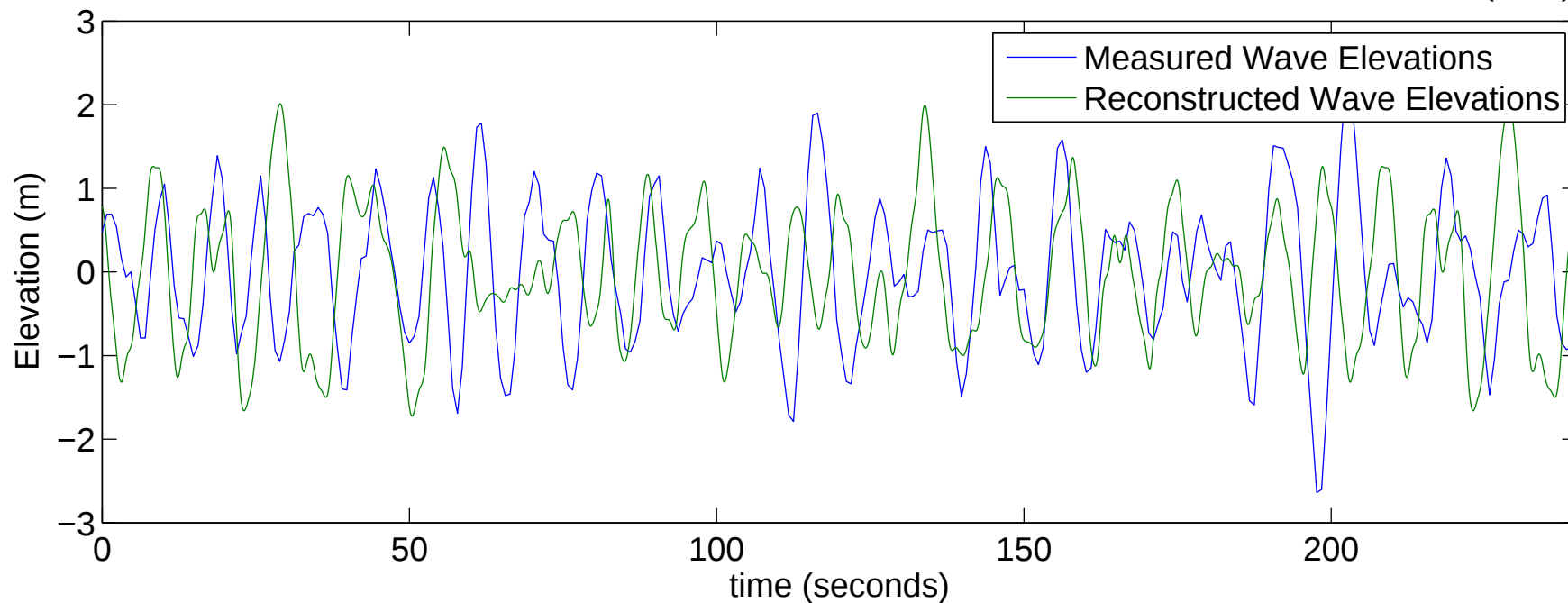
Wave conditions between November-11-2011 11:00:00 and November-11-2011 11:59:59 (PDT)
