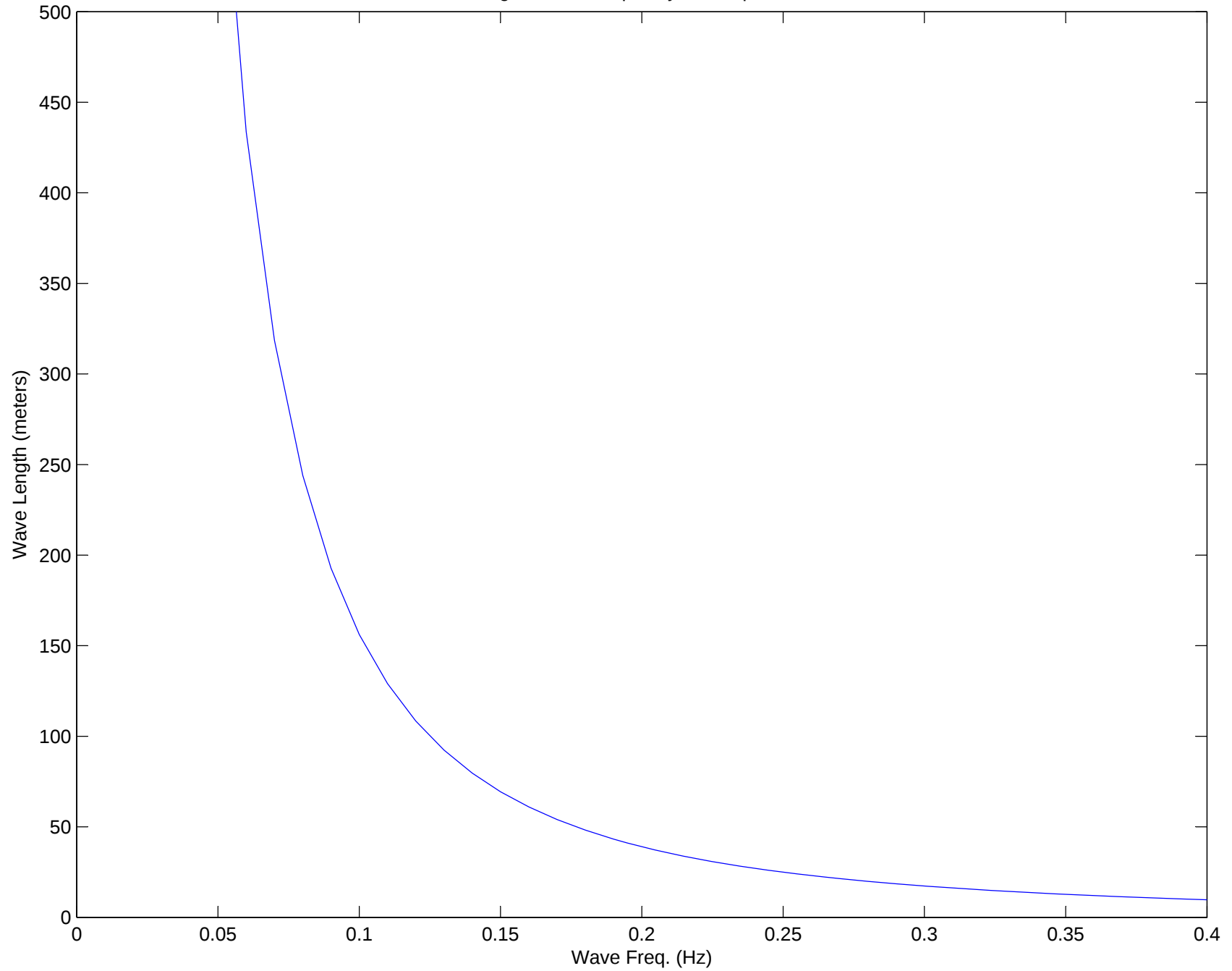
Wave length versus frequency for deep water waves
