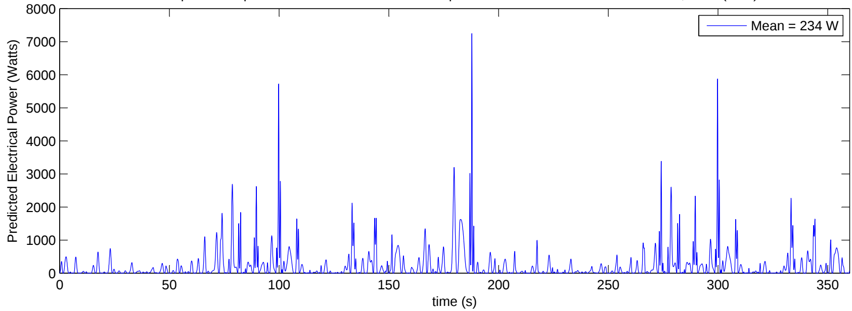
Comparison of predicted and measured electrical power for Sea State at 1600 on Nov 10, 2011 (PDT)
