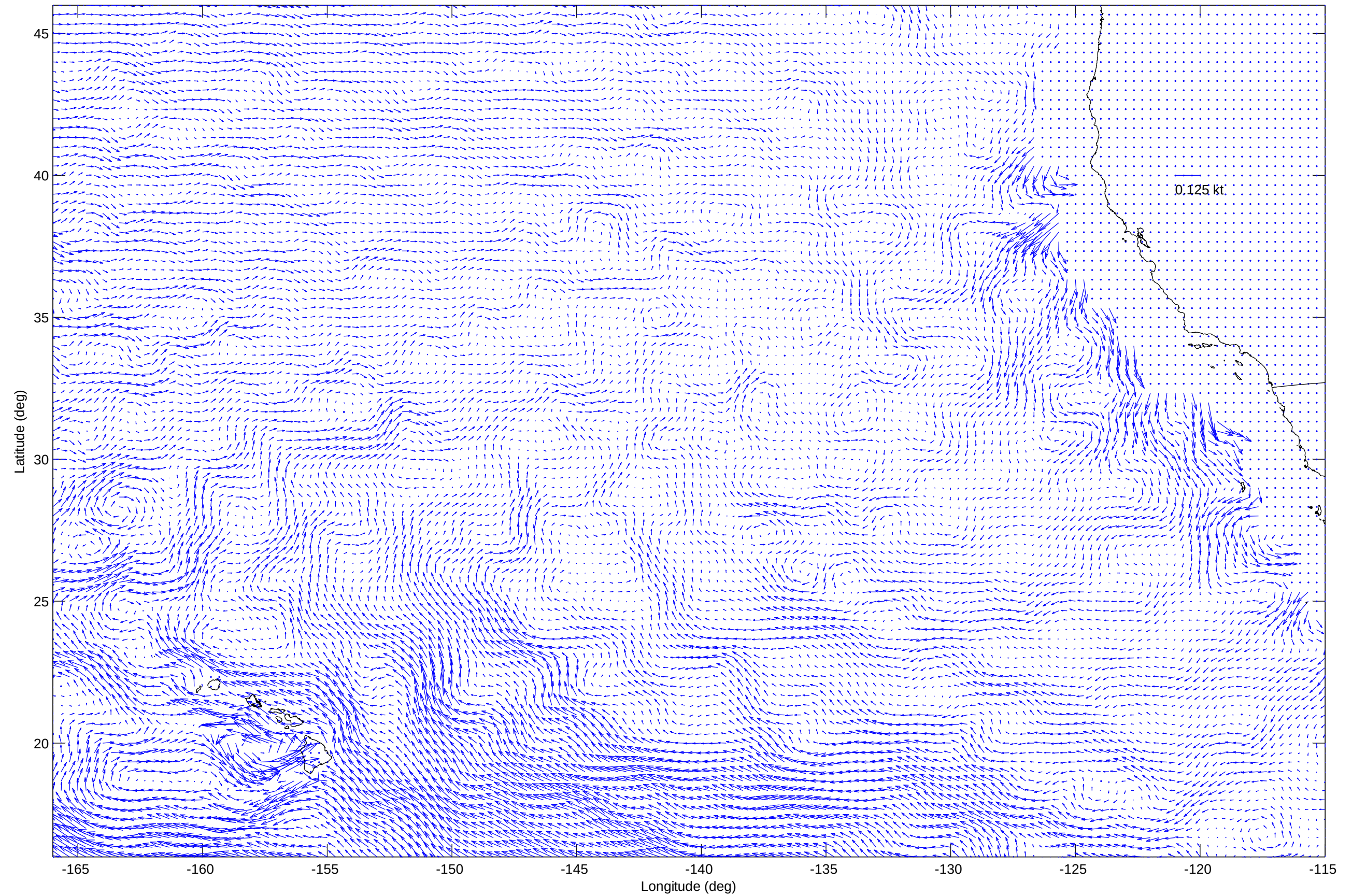
Mean June and July currents oscar_vl1992.nc - oscar_vl2014.nc
