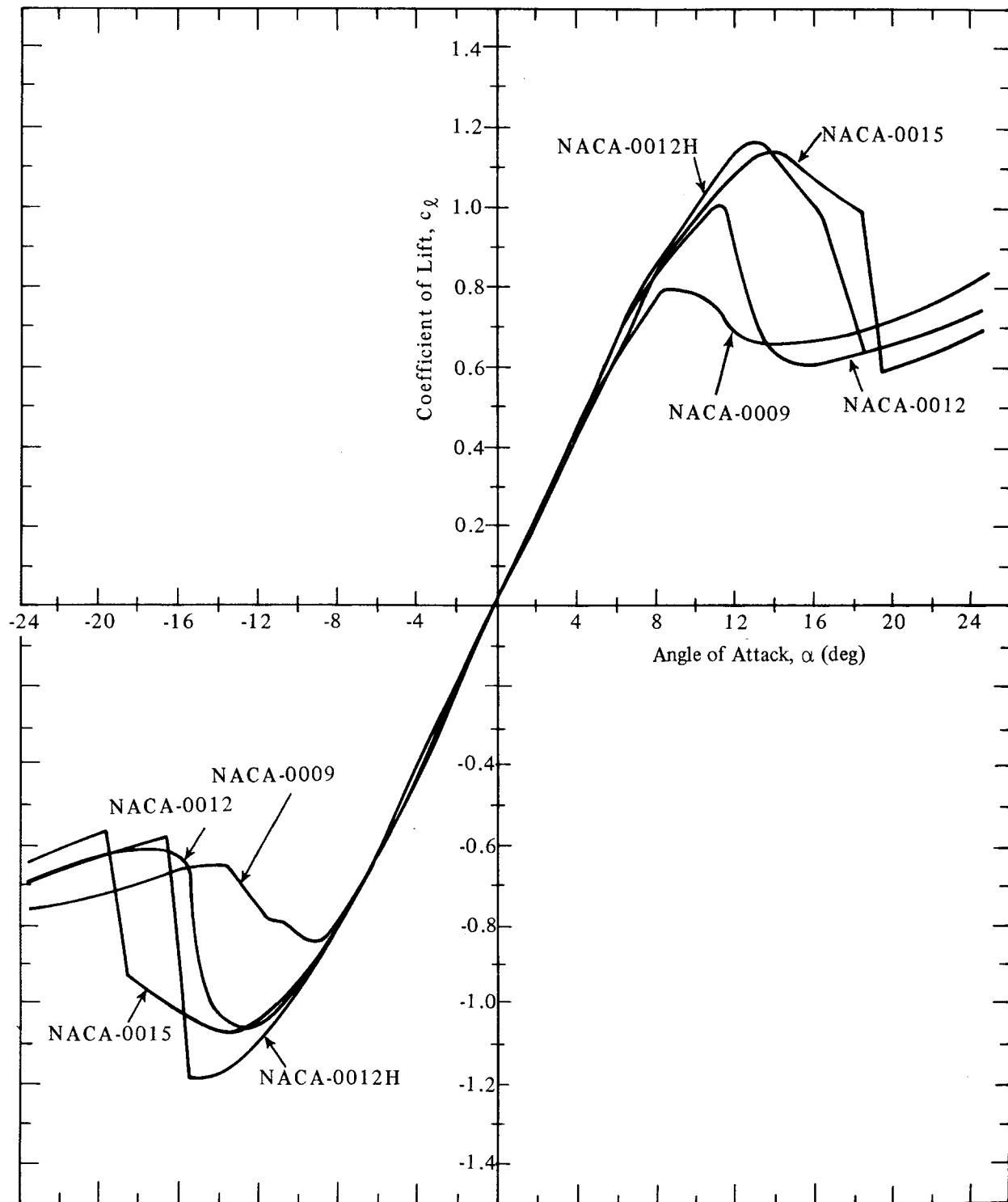
Figure 8. Section Lift Coefficients for Four Airfoil Sections at an Approximate Reynolds Number of 0.70 \times 10^6
