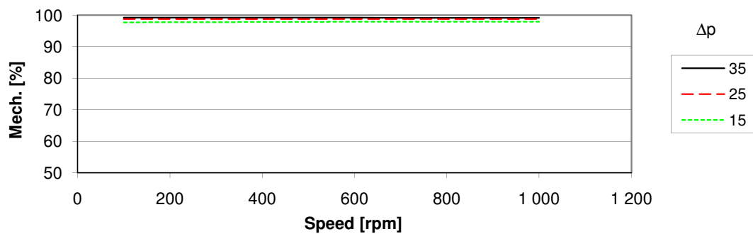
Efficiencies for F11-12 Motor
