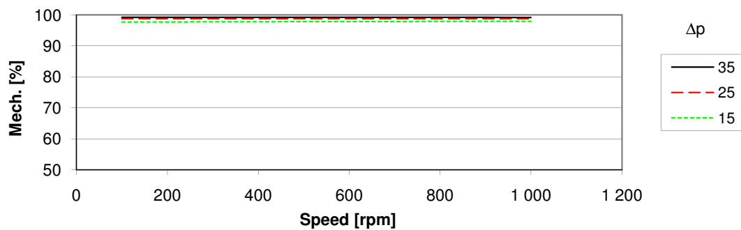
Efficiencies for F11-5 Motor
