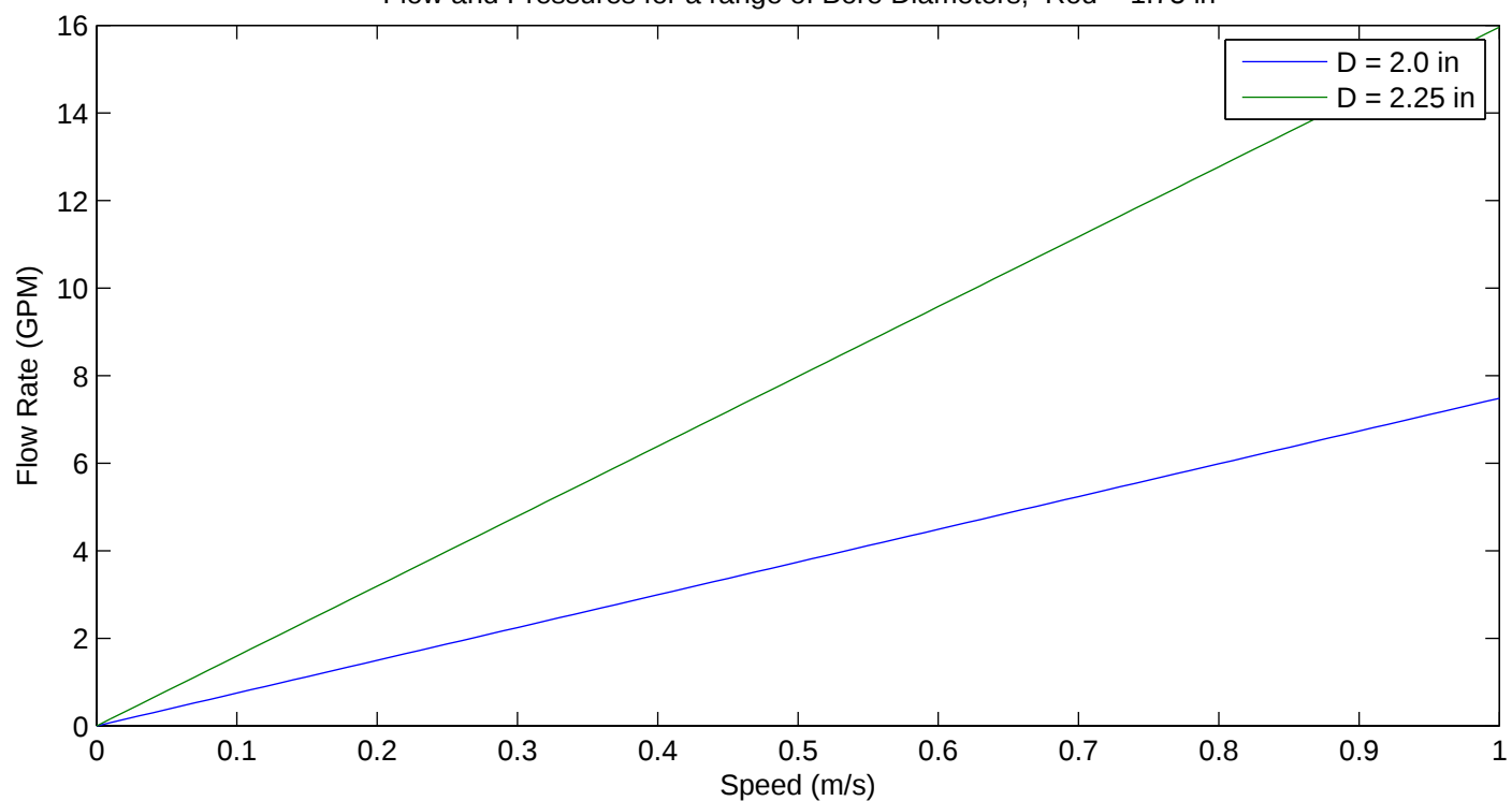
Flow and Pressures for a range of Bore Diameters; Rod = 1.75 in
