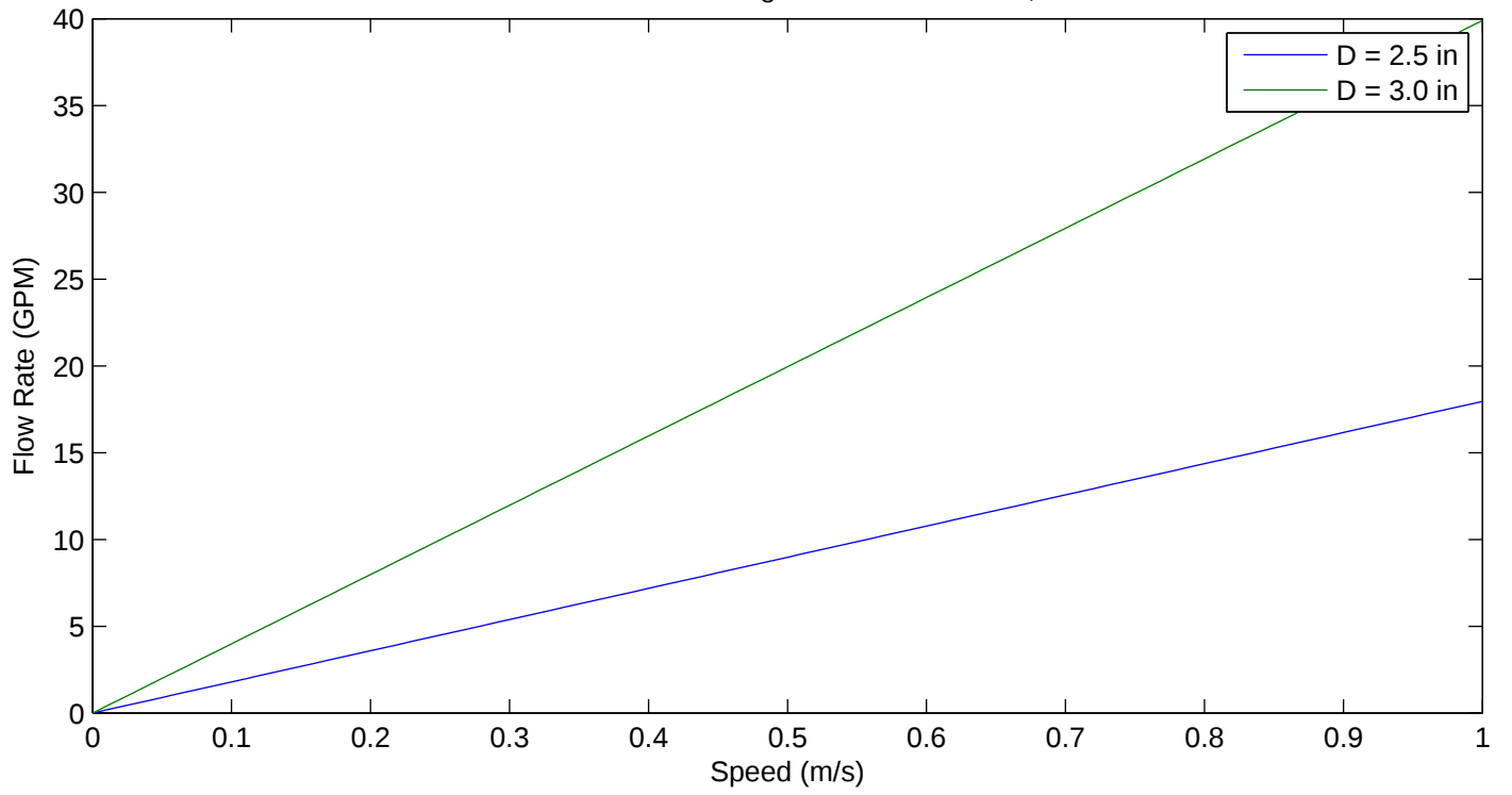
Flow and Pressures for a range of Bore Diameters; Rod = 2 in
