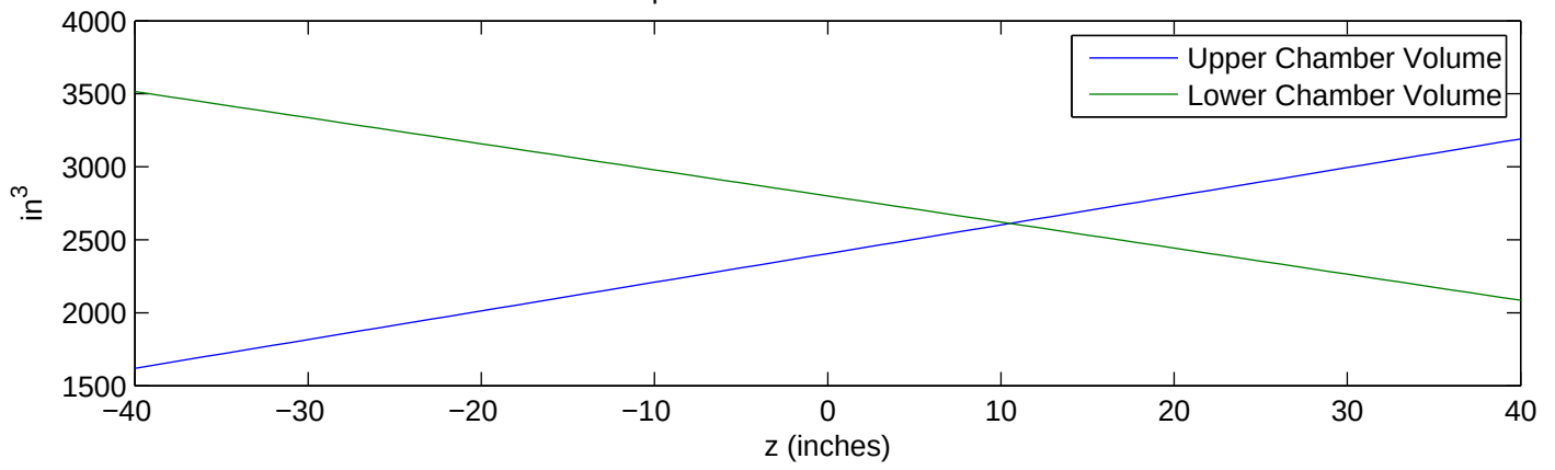
Adiabatic Compression of Diatomic Gas k = 1.8
