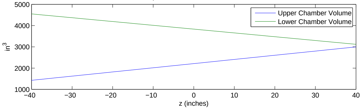
Adiabatic Compression of Diatomic Gas k = 1.820 \text{ lbs/m}
