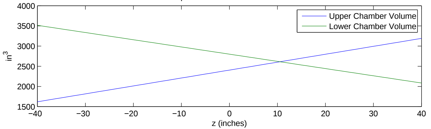
Adiabatic Compression of Diatomic Gas k = 1.9
