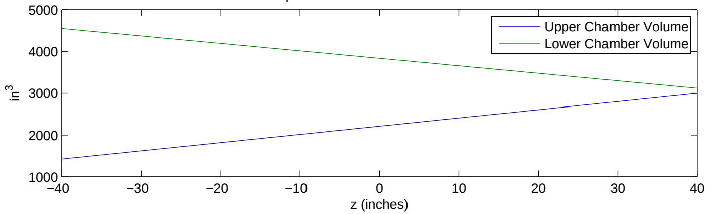
Adiabatic Compression of Diatomic Gas k = 1.927858 \text{ lbs/m}
