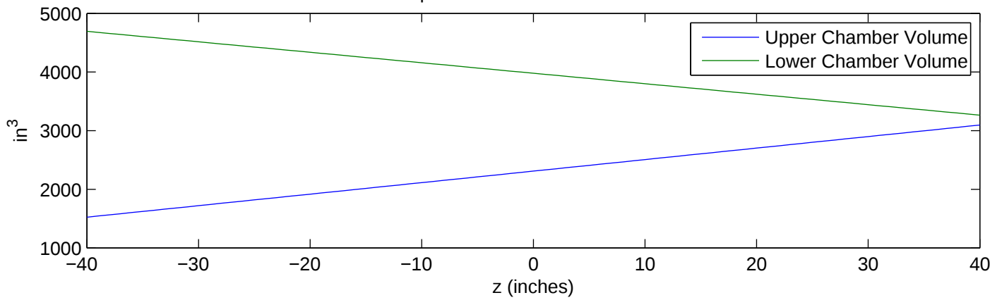
Adiabatic Compression of Diatomic Gas k = 2000\text{lbs/m}
