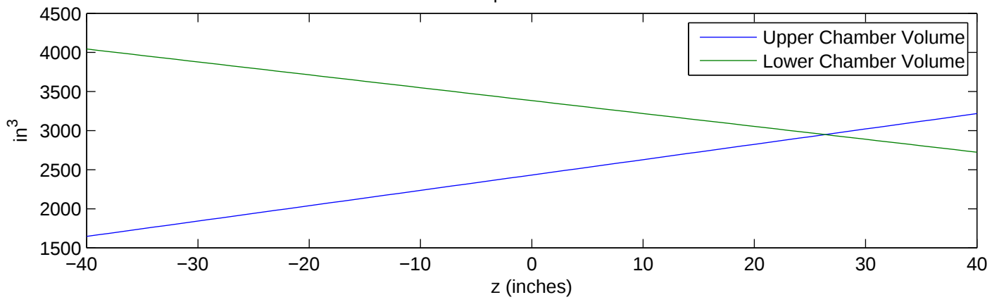
Isothermal Compression: k = 1600 \text{ lbs/m}
