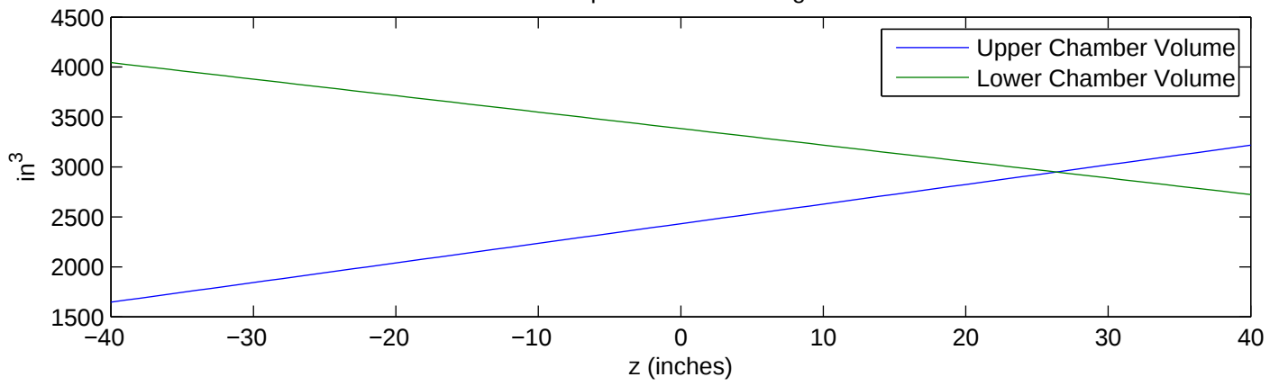
Isothermal Compression: Wet Weight = 1600 lbs
