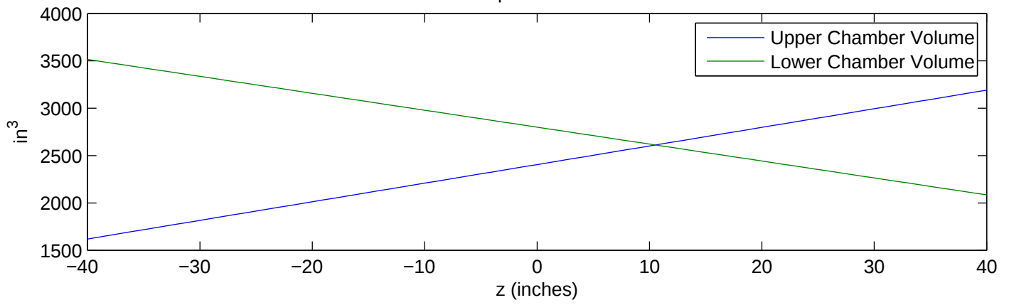
Isothermal Compression k = 1700\text{lbs/m}
