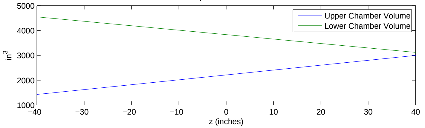
Isothermal Compression k = 1790.5959 \text{ lbs/m}
