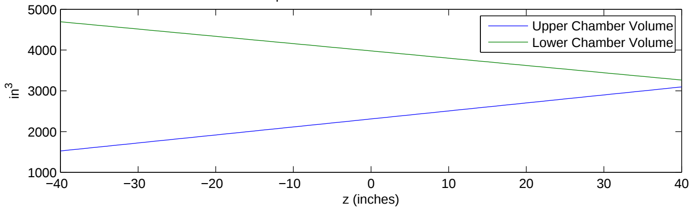
Adiabatic Compression of Diatomic Gas k = 1.8256717
