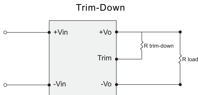
FIGURE 5: TRIM-DOWN VOLTAGE SETUP
