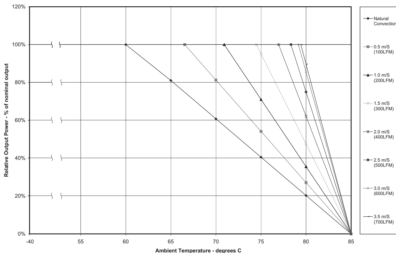
FIGURE 1. OUTPUT DERATING
