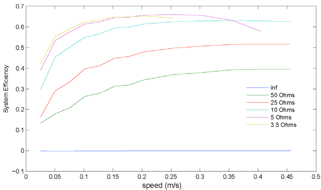
Figure 1: Conversion efficiencies of power take-off system at different speeds and electrical loadings.
