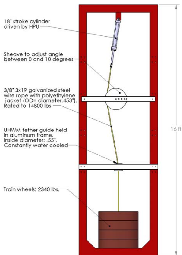
Figure 4: Tether guide test set-up.
