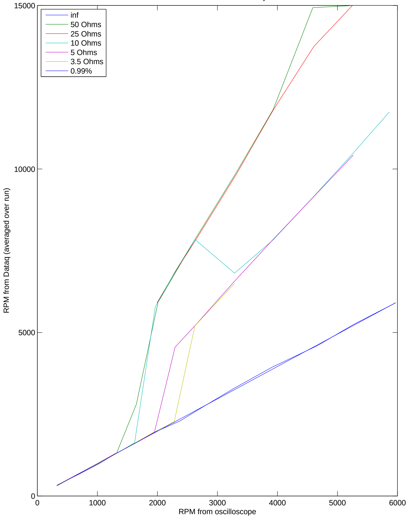
RPM Measurement Accuracy
