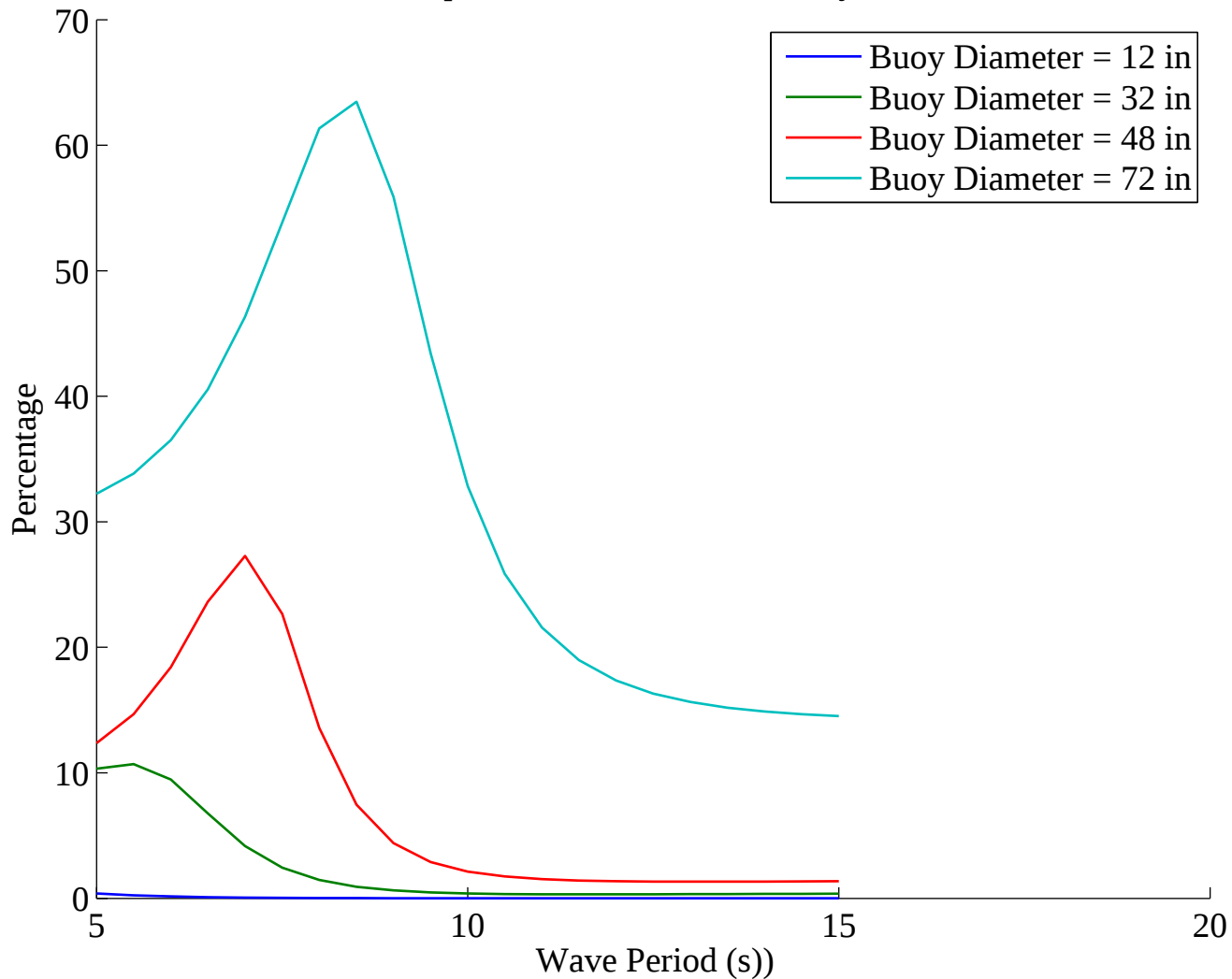
Power capture relative to 96 inch buoy reference
