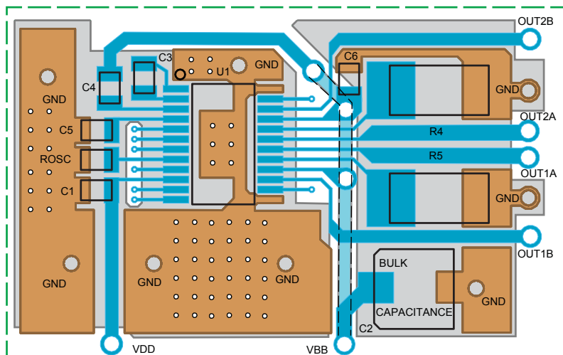
LP package typical application and circuit layout
