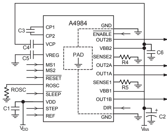
LP package typical application and circuit layout
