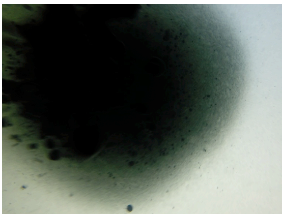
Figure 6.1.4 Upward looking photos of the spill under nilas (left) and frazil (right) at HSVA. Oil can be identified by its contrast with the clean ice around it, but for the oil encapsulated within the frazil, the more greyish color suggests that under ice of variable thickness discrimination of the encapsulated oil from thick ice or ice with a thick snow cover may be more difficult. These photos were taken in ambient light
