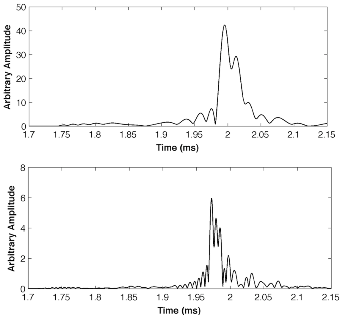
Figure 5.1.1 Backscattered pulse compressed output for 160 kHz (top) and 500 kHz (bottom) signals from the basal ice layer prior to oil release. The ice bottom is located at 1.96-1.98 ms (the two traces were taken two hours apart), corresponding to a range of 1.41 – 1.43 m. The ripples ahead of the main peak are due to side lobes and/or effects of the matched filter processing. More structure after the ice/water interface is visible after the main peak.
