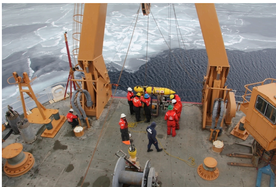
Figure 3.2.1 A-frame on stern of the Healy viewed from adjacent to the vehicle conning station. This was used to deploy the AUV as the port crane reportedly was not working properly and the starboard crane was used for other operations during the exercise. Nilas (thin grey ice < 10 cm thick) and broken ice were frequently present off the stern so that the AUV was often deployed and recovered amongst ice.
