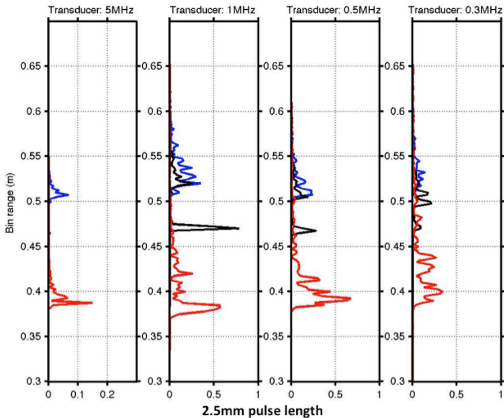
Figure 5.3.1 echograms for the Aquascats transducers in the SAMS Tank 1 tests at frequencies of 5, 1, 0.5, and 0.3 MHz, from left to right for a pulse length of 2.5 mm. Range is on the vertical axis, with the original water/air interface at about 0.6m before ice growth began. The blue trace shows the scattering after about 7 cm of growth. The Black trace is immediately after oil is deployed, and the red trace is the response after encapsulation within ~15 cm of ice after 9 days. Range uses a nominal sound speed of 1500 m/s. The difference is not significant for water or oil, but is for ice (sound speed unknown), so the ranges are not true ranges.
