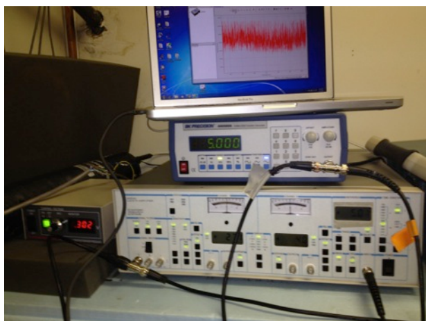
Figure 4.1.2 Laser fluorometer bench set-up. This includes a lock-in amplifier to detect the signal (bottom), a signal generator to modulate the laser (middle), and the power supply for the PMT (left). The laptop on top displays the USB4000 spectral response. In this case, there is no oil deployed, and so the returned spectrum is very nearly white noise, as expected.
