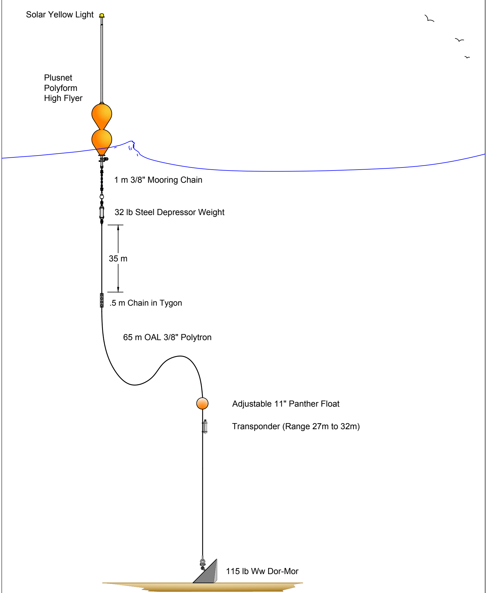
High Flyer Transponder Mooring 54-64 meter Depth Range
