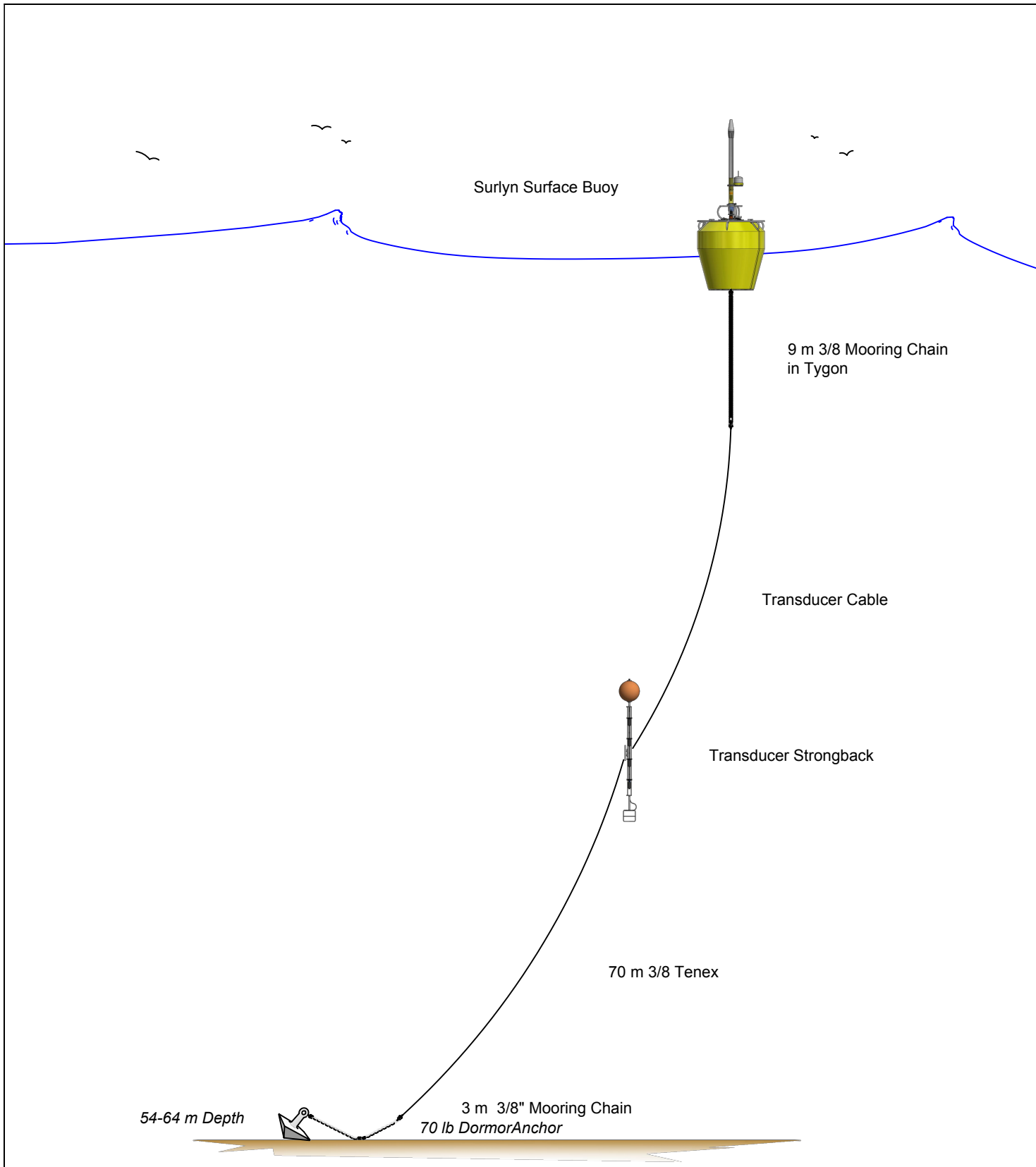
Modem Buoy with Transducer Mooring
