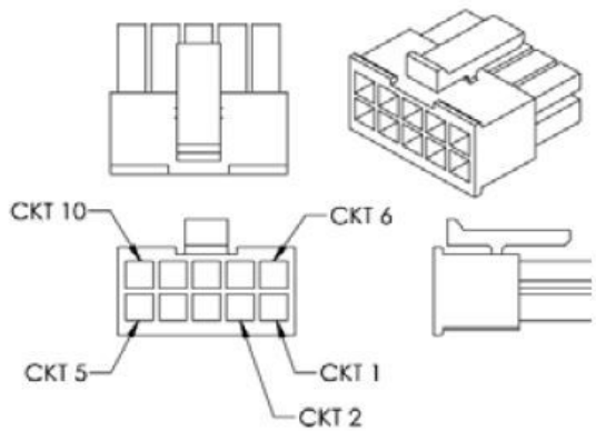
WIRE SIDE P1
