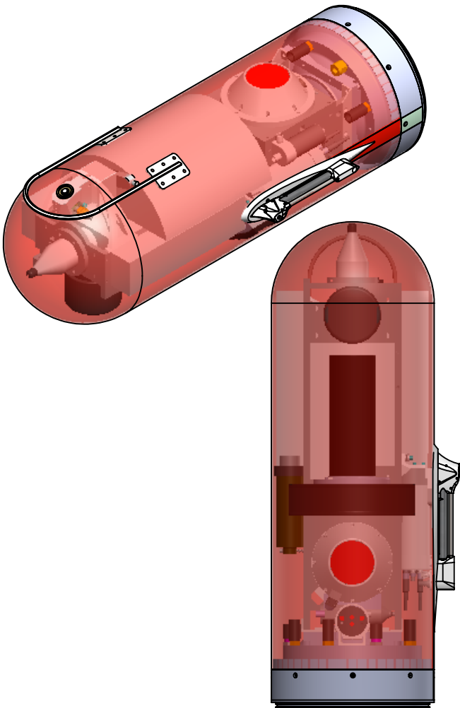
Config 4 Seafloor Mapping Multibeam, INS, Tall antenna, Soundscape
