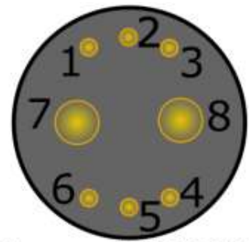
Seacon MINK-8/L
