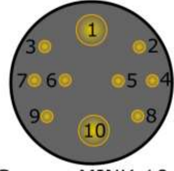
Seacon MINK-10/L
