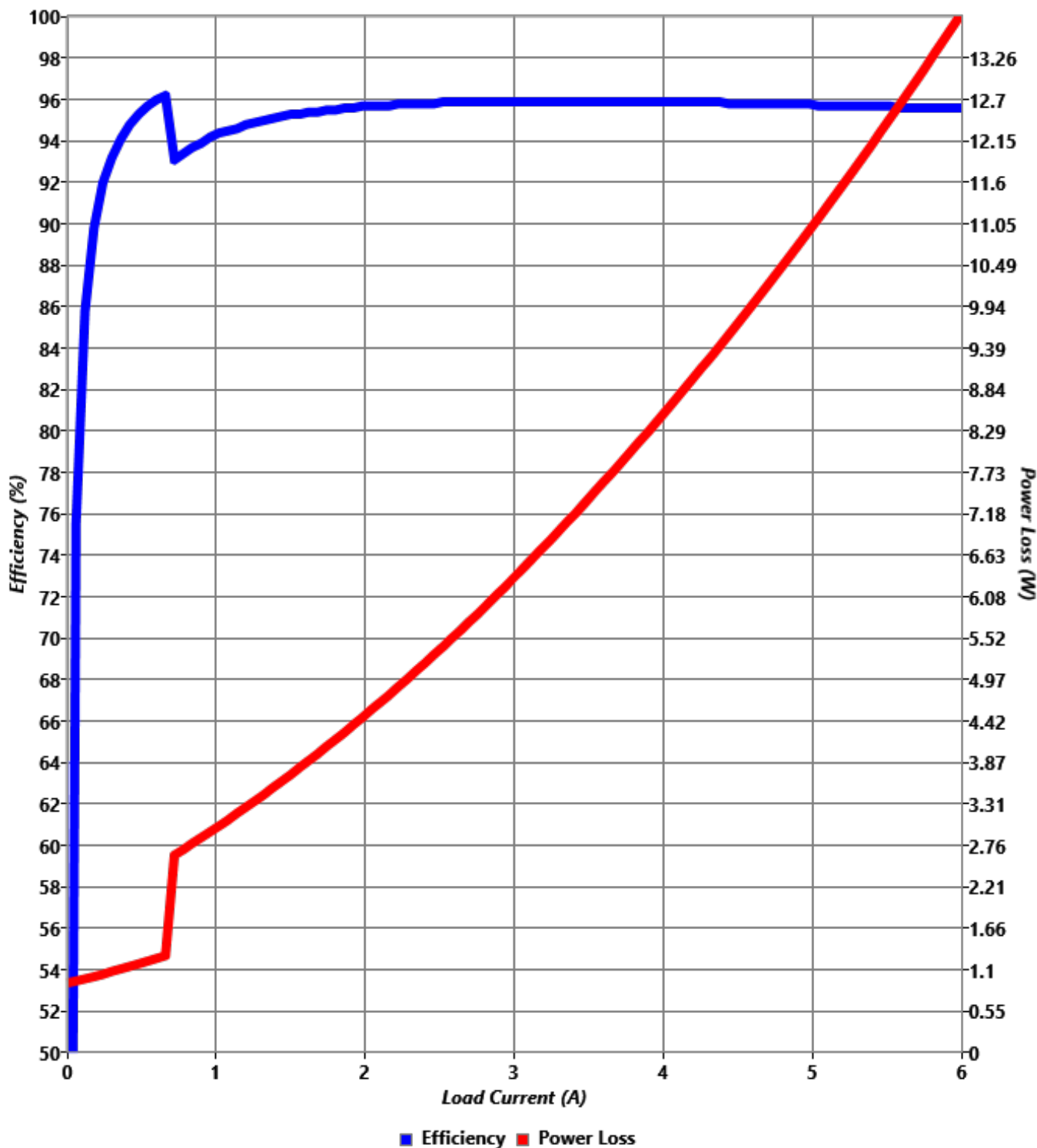
Rail #1 (48.31V) Efficiency & Power Loss
