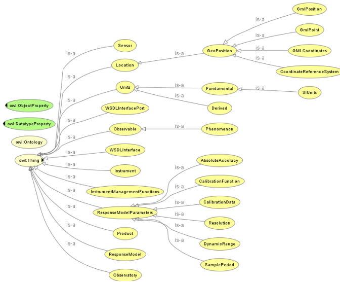
Fig. 5. Some of the OWL classes used to describe a CIMA instrument
