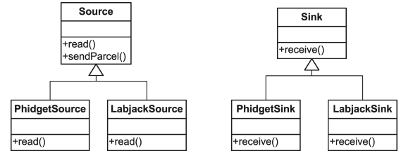
Fig. 6. Source and Sink classes
