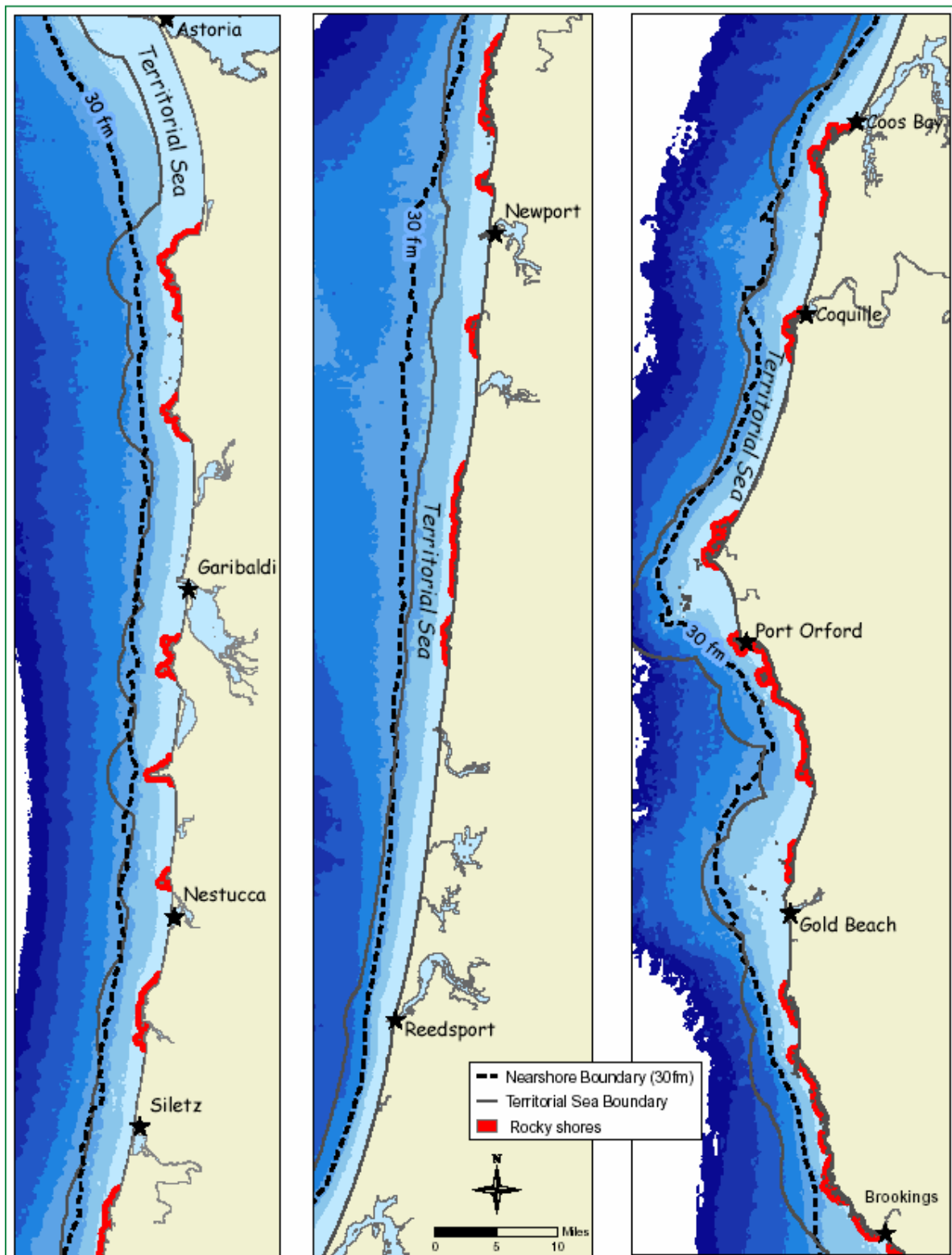
Figure 3.1 Oregon's nearshore ocean showing the 30-fathom depth contour and the 3-nautical mile demarcation of the Territorial Sea (ODFW Nearshore Team 2006). Read areas are rocky shore habitats; areas not blocked in red are sedimented shorelines.
