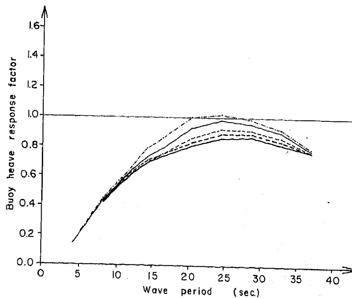
FIG. 4. As in Fig. 3, but without damping plate. Wave amplitudes as in Fig. 5.
