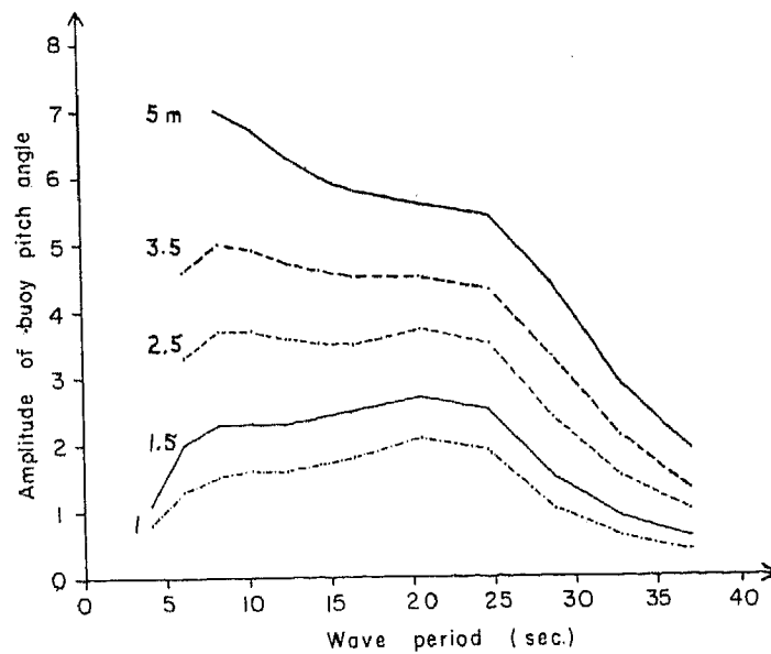
FIG. 5. Pitch response of the buoy. The presence of the damping plate does not affect the results. Wave amplitudes in meters are shown close to each line.
