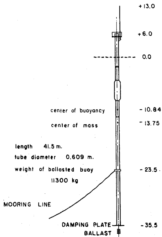
FIG. 1. Buoy configuration—main characteristics are given in Table 1, dimensions in meters.
