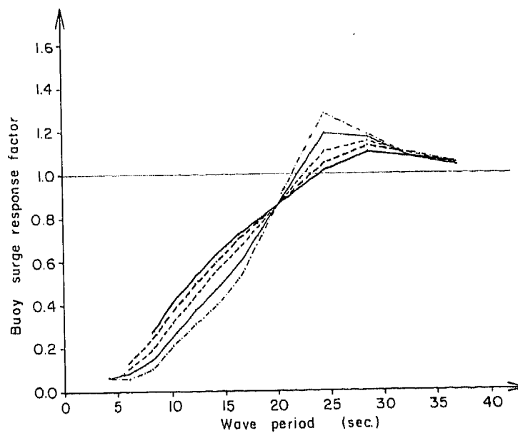
FIG. 6. Surge response factor (surge amplitude/wave amplitude) of the buoy. The presence of the damping plate does not affect the results. Wave amplitudes as in Fig. 5.
