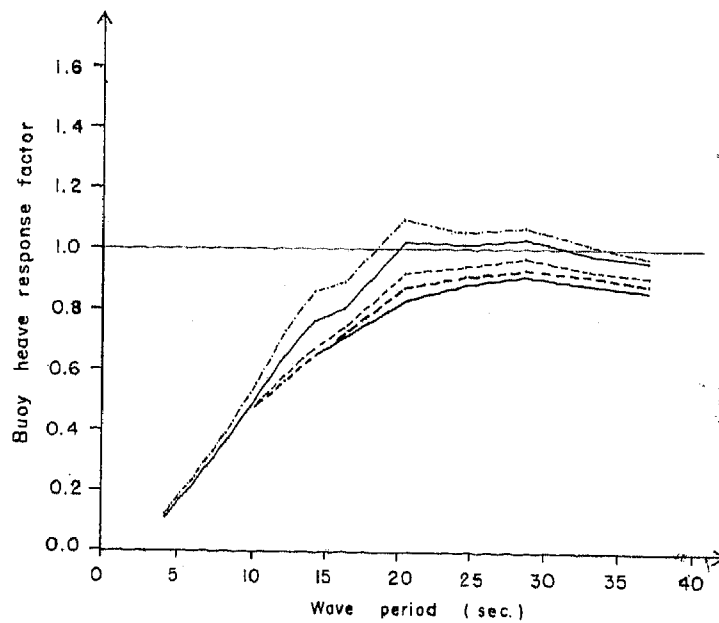
FIG. 3. Heave response factor (heave amplitude/wave amplitude) of the buoy, with damping plate. Wave amplitudes as indicated in Fig. 5.
