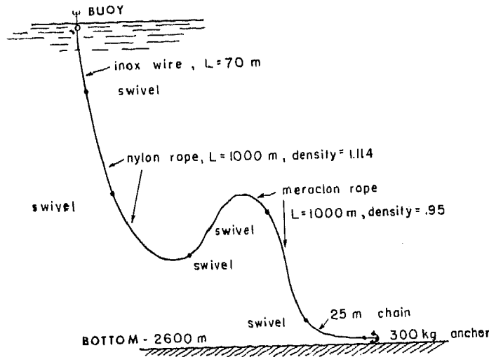
FIG. 2. Mooring arrangement in 2600 m depth.
