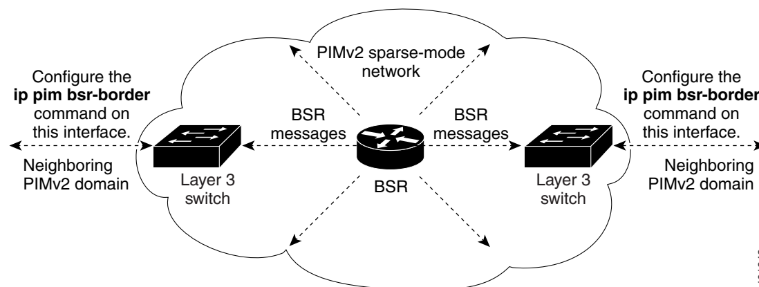
Figure 36-3 Constraining PIMv2 BSR Messages
