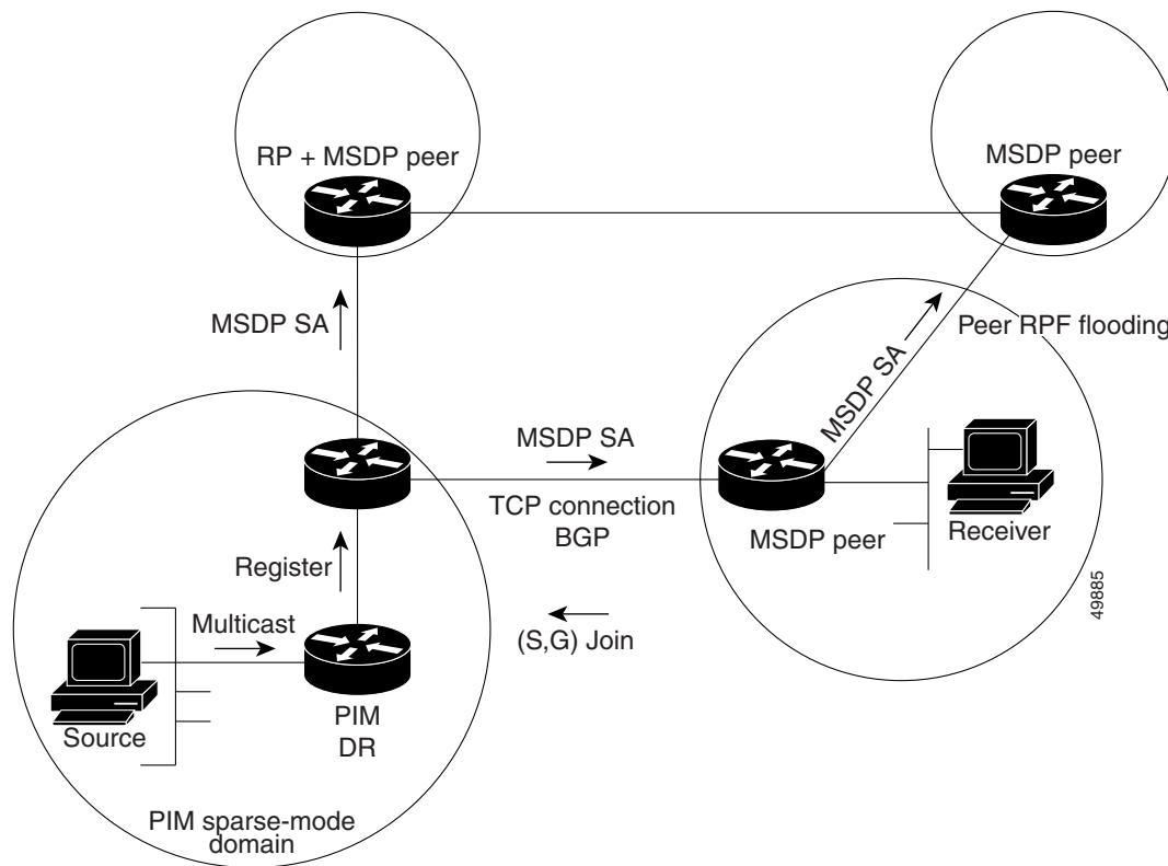
Figure 37-1 MSDP Running Between RP Peers
