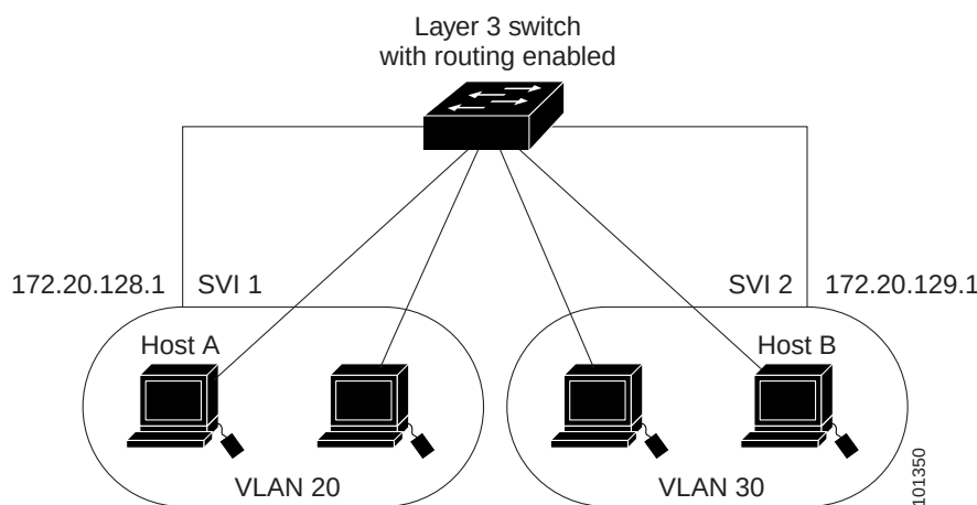
Figure 11-1 Connecting VLANs with the Catalyst 3750 Switch
