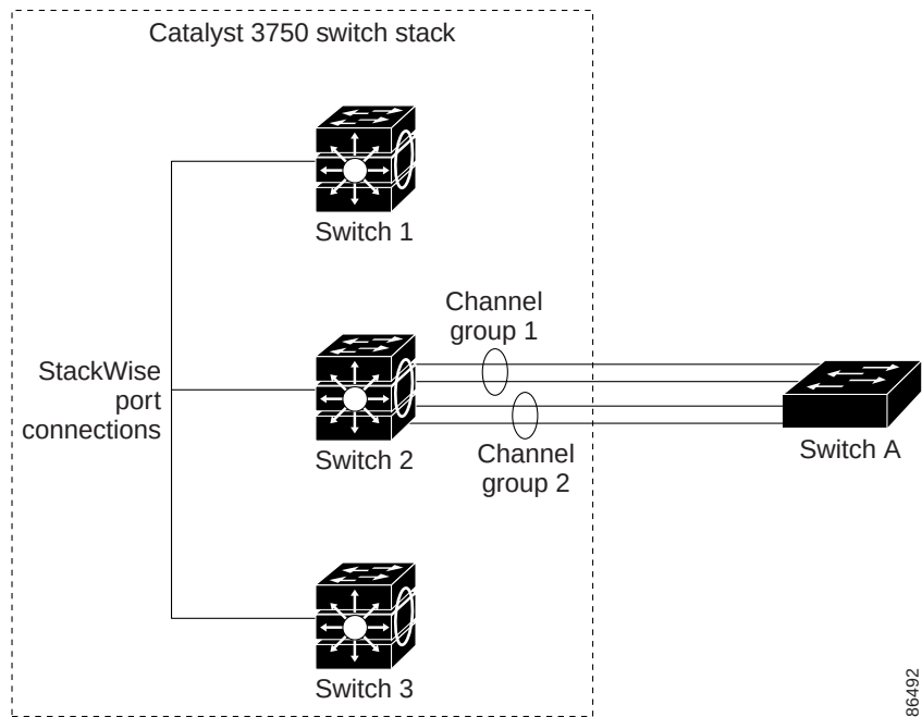
Figure 34-2 Single-Switch EtherChannel
