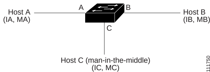
Figure 23-1 ARP Cache Poisoning
