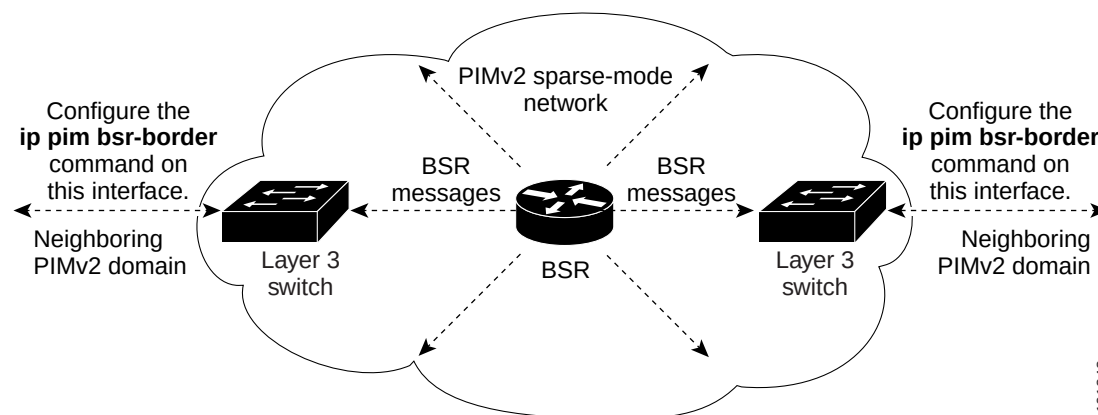
Figure 38-3 Constraining PIMv2 BSR Messages
