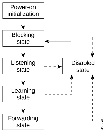
Figure 18-2 Spanning-Tree Interface States
