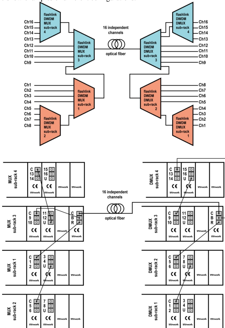
Figure 2.8: 16-channel unidirectional DWDM system, description of system and connections of the sub-racks 1,2,3 and 4.
