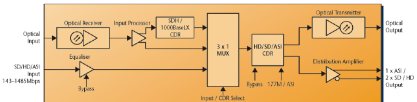
Figure 1 - MR-TR-D15xx Multi Rate Transponder for DWDM
