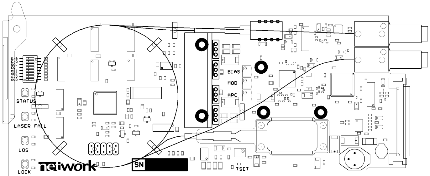
Figure 2 - MR-TR-D15xx board layout.
