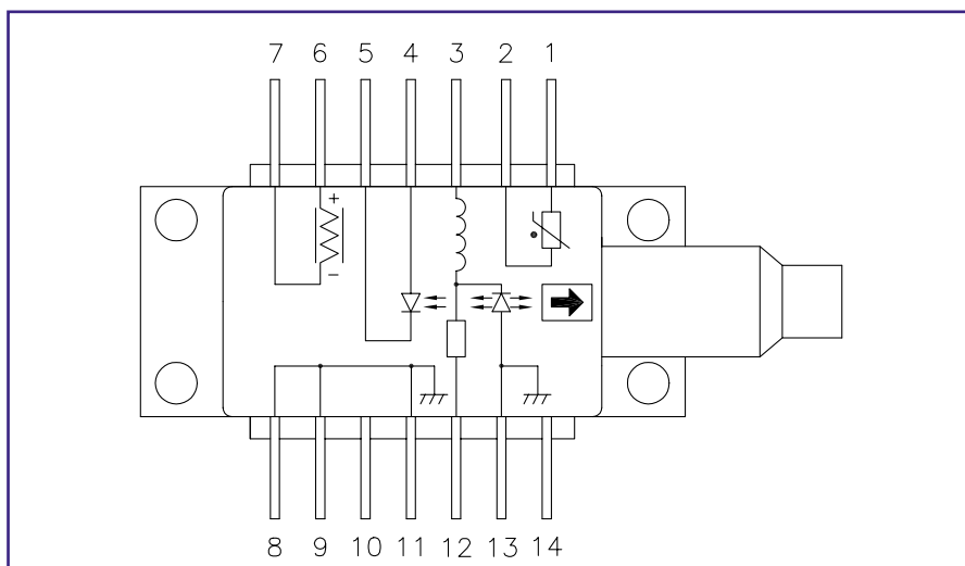
Figure 1: Schematic diagram
