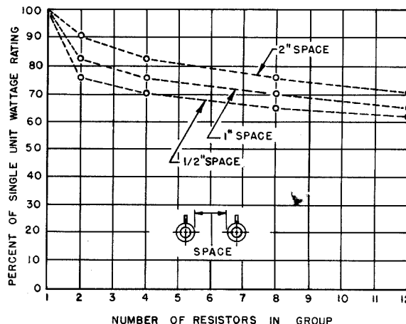
Fig. 11: Derating of Resistors to Allow for Grouping.
