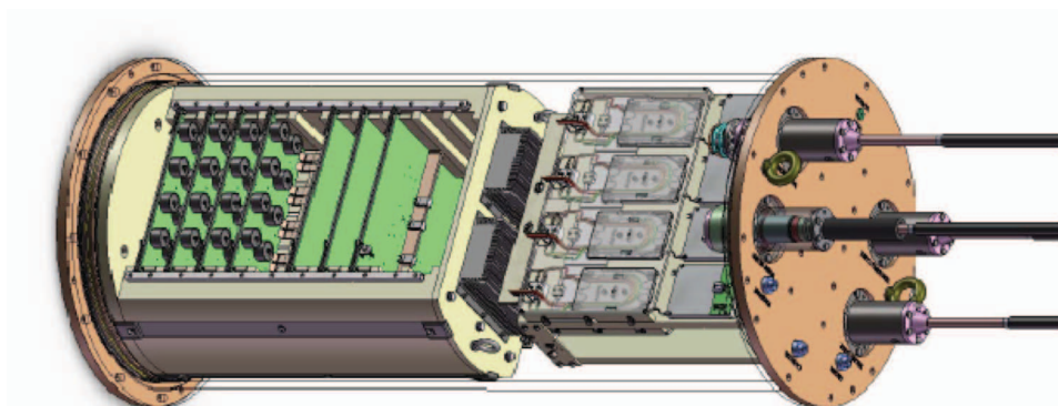
Figure 3. Primary node solid model with MVC on left and optical payload on right
