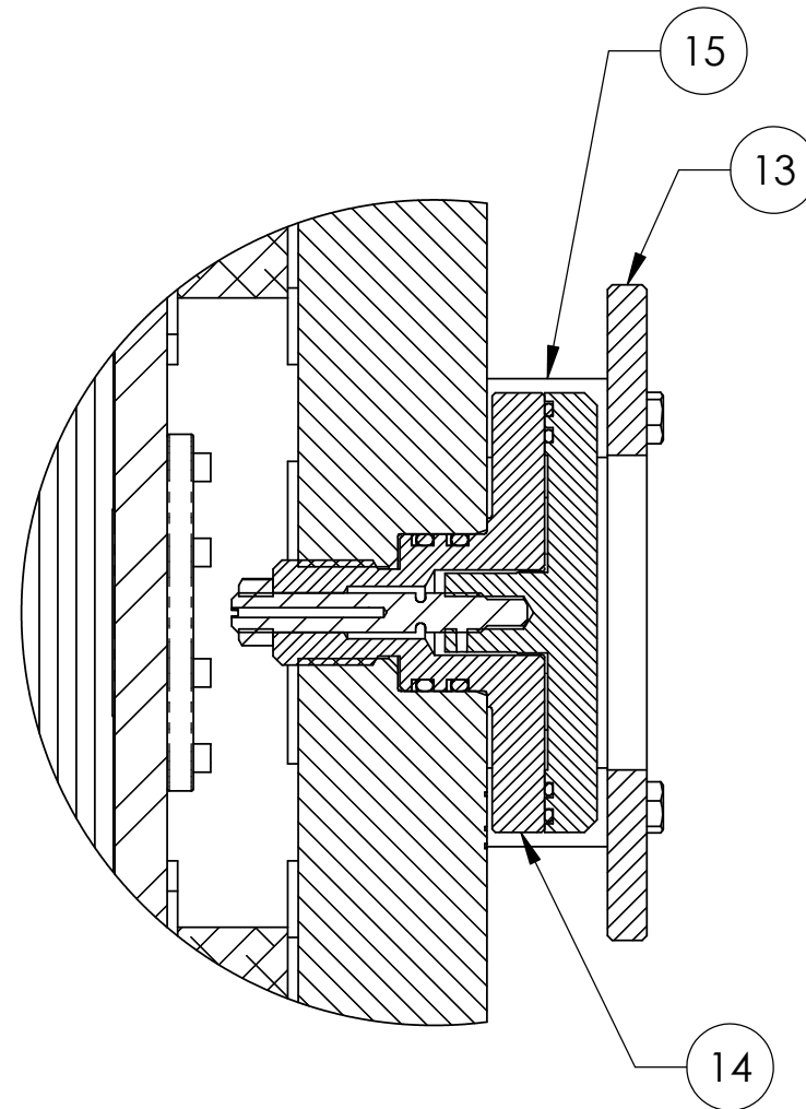
SECTION F-F SCALE 1 : 2
