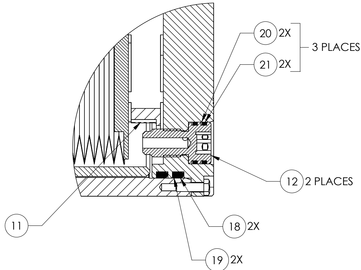
DETAIL D SCALE 1 : 2
