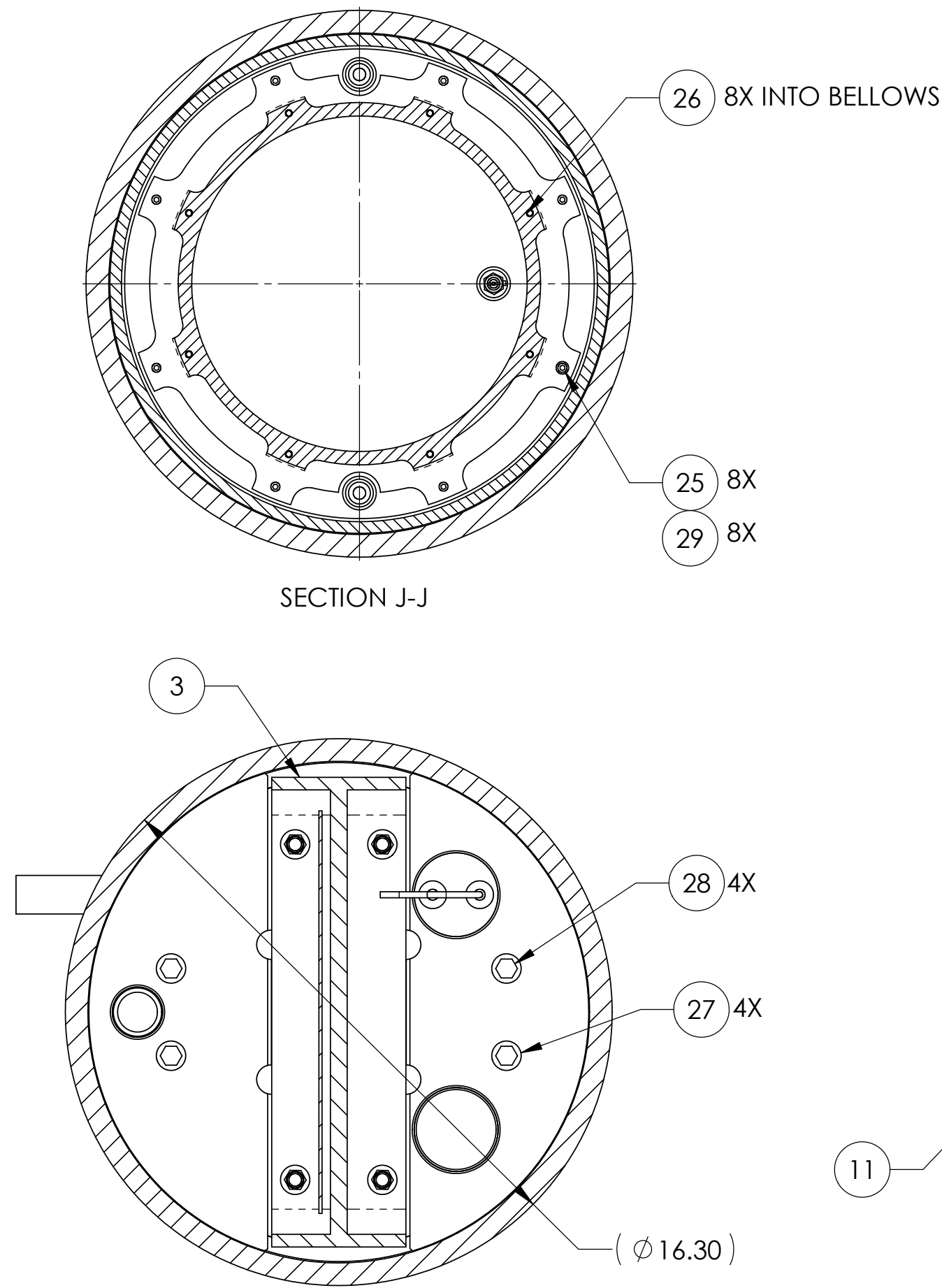
SECTION B-B
