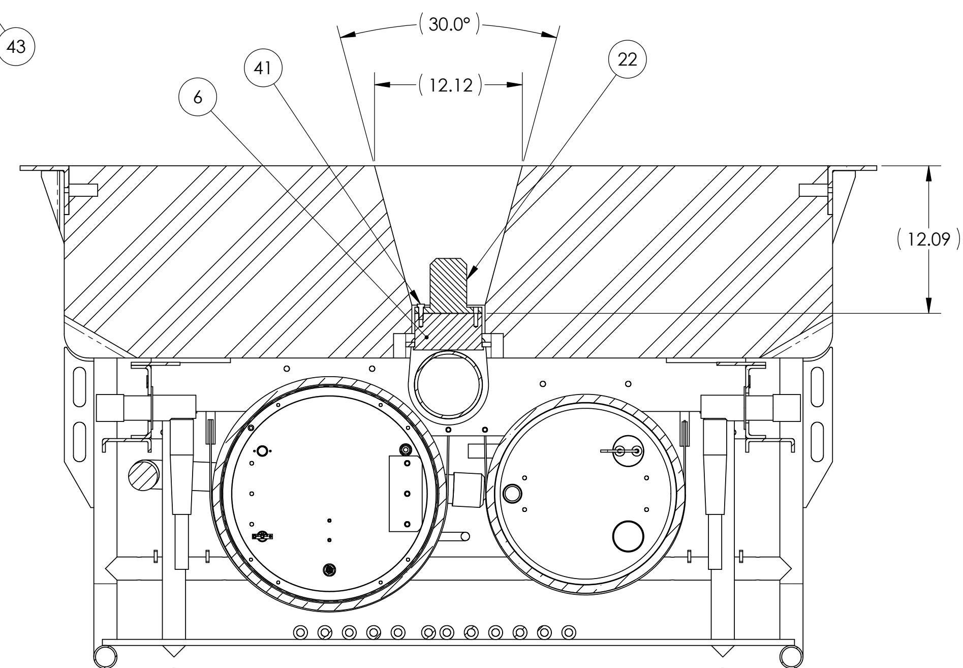
SECTION C-C
