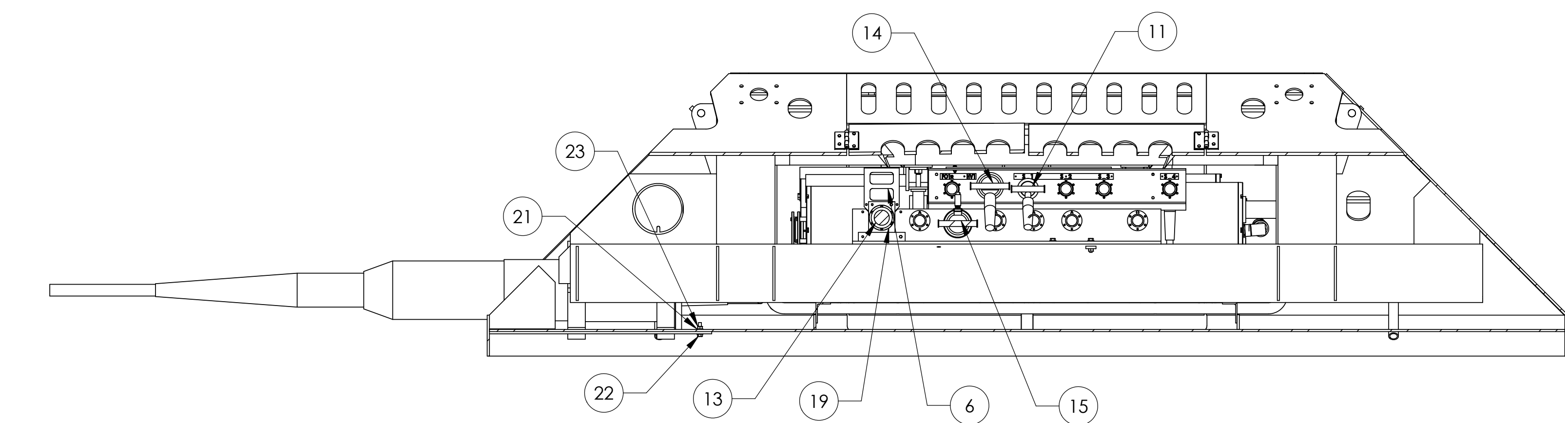
SECTION B-B
