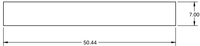
8 110434-74 TRF OUTSIDE SKIRT CABLE END MATERIAL: A-36 3/8 THK. NO. REQ'D: 2
