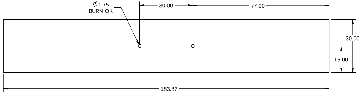
10 110434-72 TRF GROUND SKIRT PLATE MATERIAL: A-36 3/8 THK. NO. REQ'D: 2
