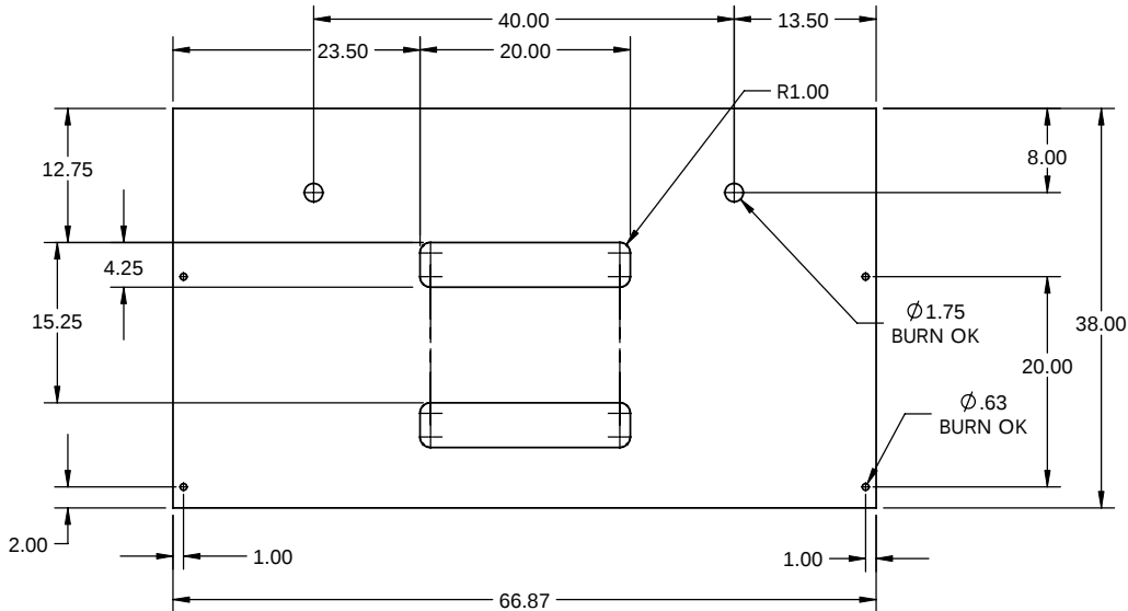
23 110434-53 TRF CTA MUD MAT END MATERIAL: A-36 3/8 THK. NO. REQ'D: 1
