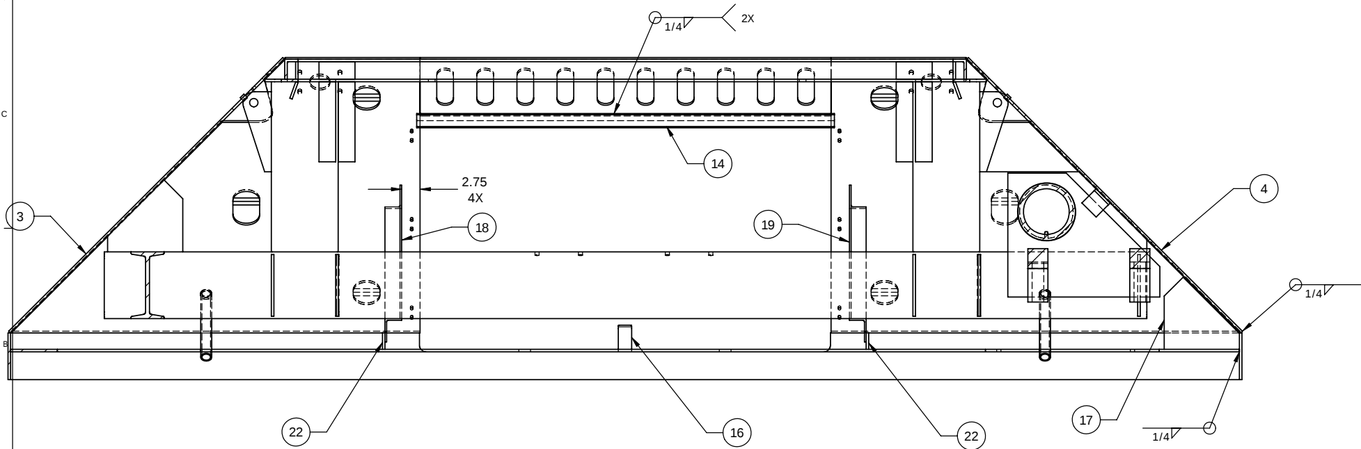
SECTION F-F SCALE 1 : 10
