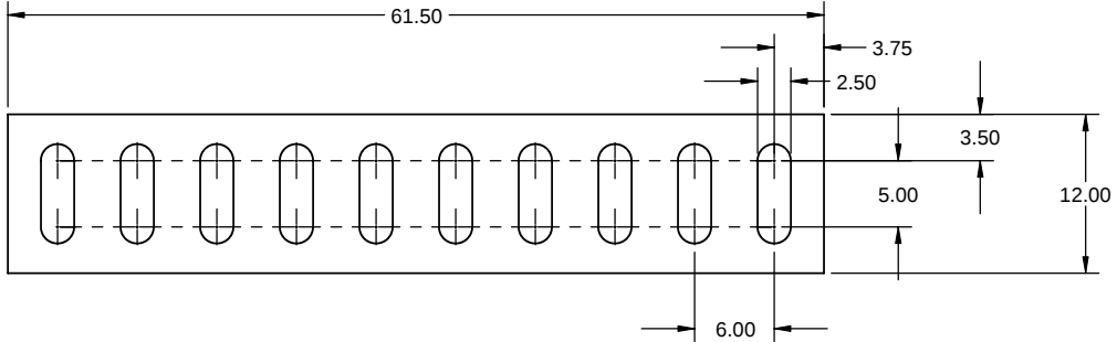
5 110434-77 VENT PLATE, TRF MATERIAL: A-36 3/8 THK. NO. REQ'D: 2
