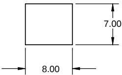
9 110434-73 TRF SKIRT PLATE SMALL MATERIAL: A-36 3/8 THK. NO. REQ'D: 2
