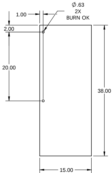
12 110434-70 TRF GROUND SKIRT CABLE END LG MATERIAL: A-36 3/8 THK. NO. REQ'D: 2
