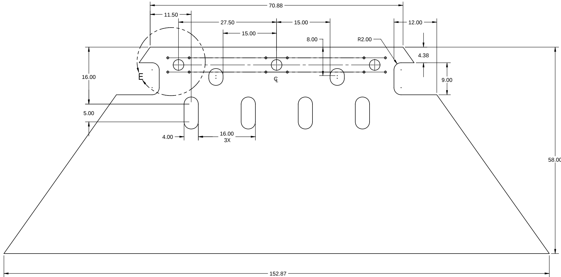
3 110434-79 TRF OUTSIDE PLATE AFT MATERIAL: A-36 3/8 THK. NO. REQ'D: 1
