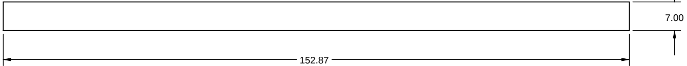
6 110434-76 TRF OUTSIDE SKIRT ANCHOR END MATERIAL: A-36 3/8 THK. NO. REQ'D: 1
