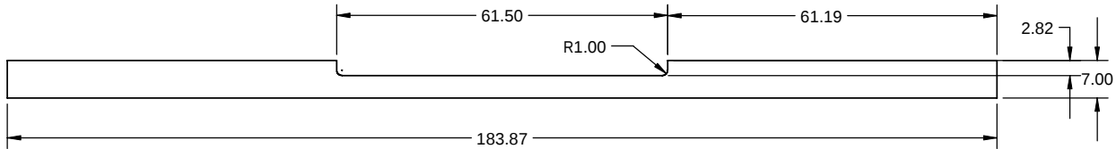
7 110434-75 TRF OUTSIDE SKIRT PLATE MATERIAL: A-36 3/8 THK. NO. REQ'D: 2
