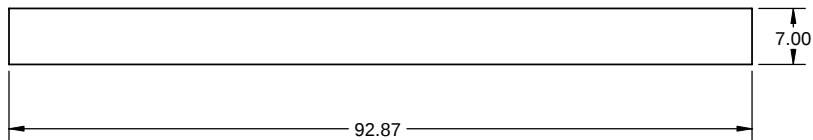
11 110434-71 TRF GROUND SKIRT END MATERIAL: A-36 3/8 THK. NO. REQ'D: 1
