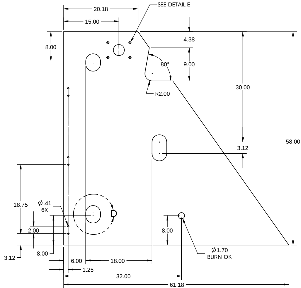
2 110434-80 TRF OUTSIDE CORNER PLATE MATERIAL: A-36 3/8 THK. NO. REQ'D: 4
