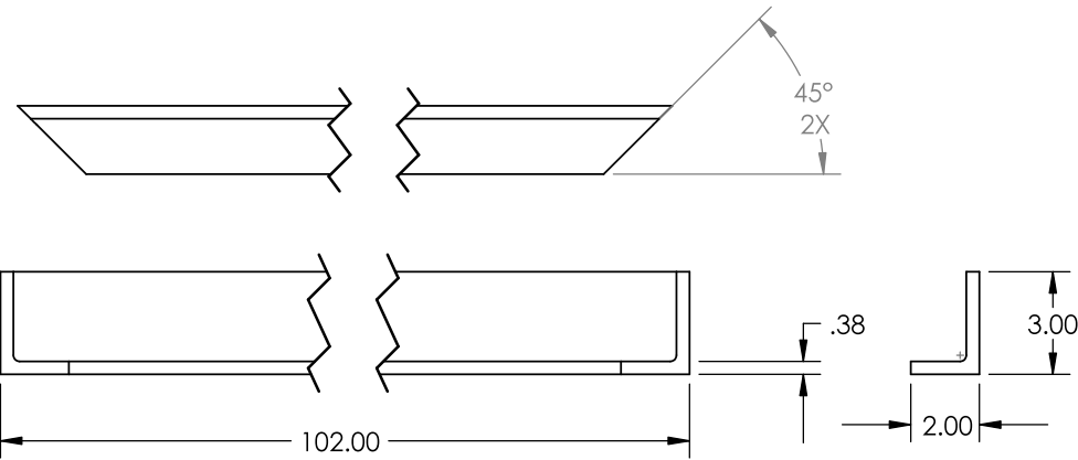
1 110434-96 MATERIAL: A-36 L 3 X 2 X 3/8 REQ'D:2
