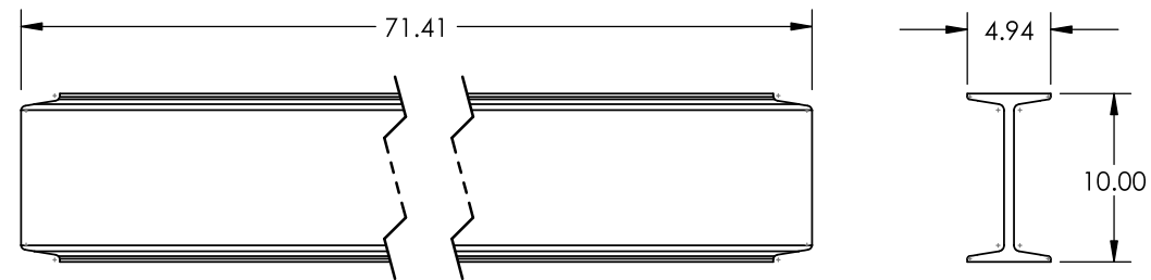
7 110434-91 MATERIAL: A-36 S BEAM S10 X 35.0 REQ'D:1
